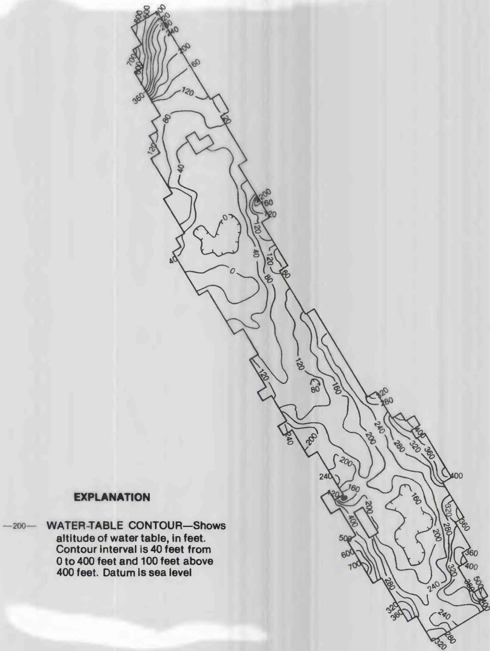
FIGURE 31A.—Spring 1961 water-table altitude.
