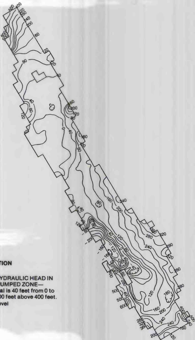
FIGURE 31B. —Spring 1961 hydraulic head in the lower pumped zone.
