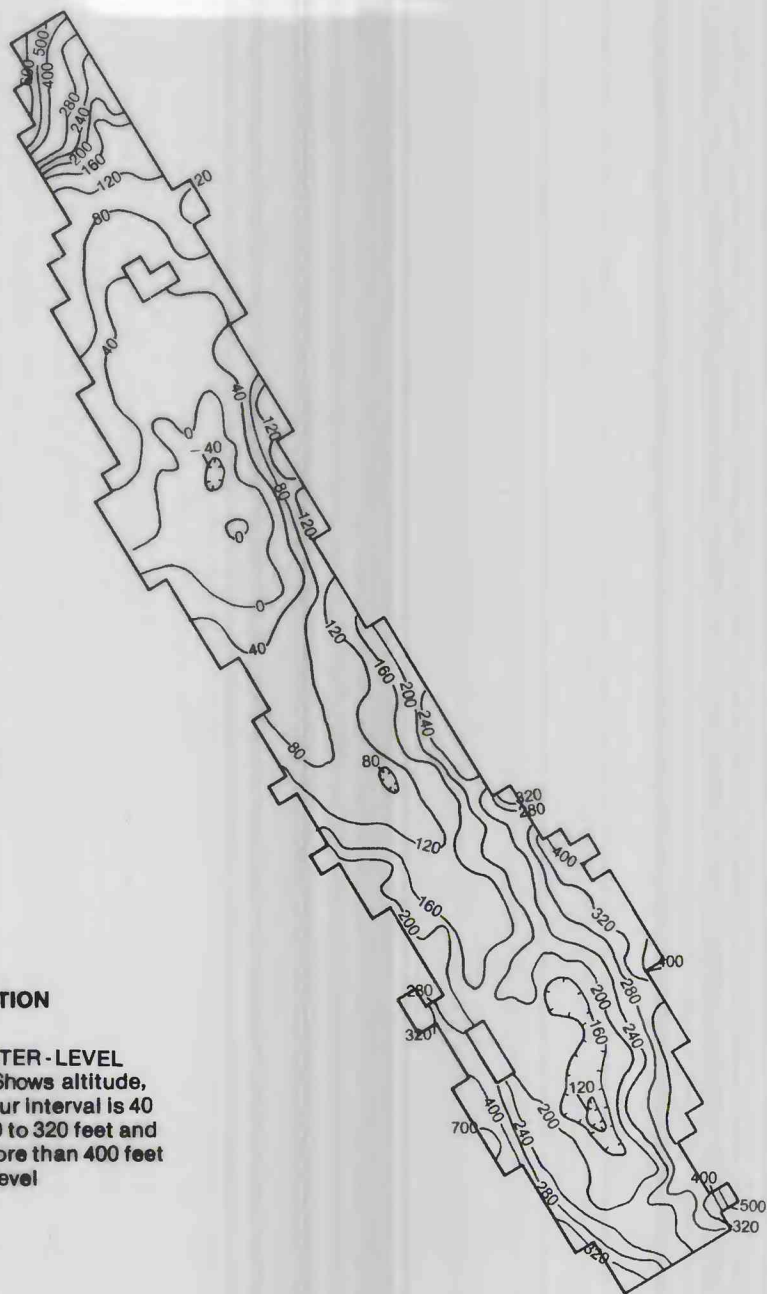
FIGURE 33A.—Observed water-table altitude, spring 1976.
