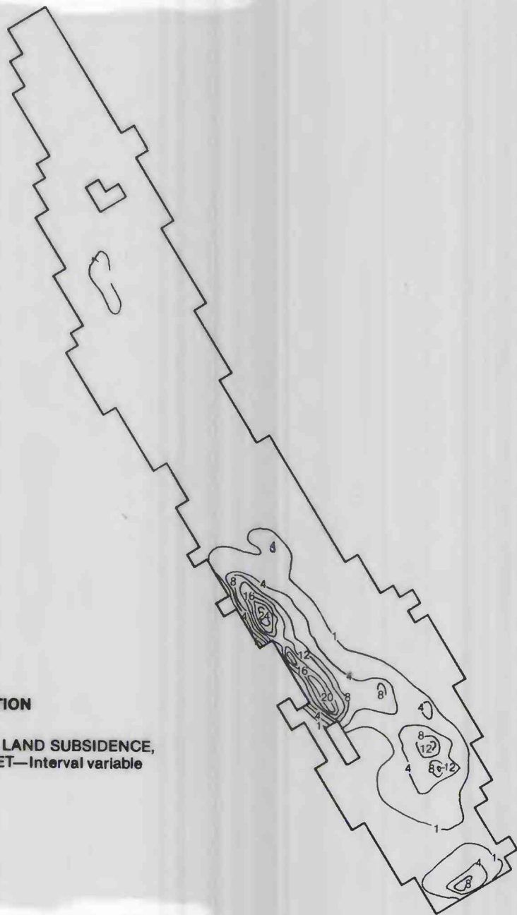
FIGURE 36B.—Land subsidence, 1926-70.
