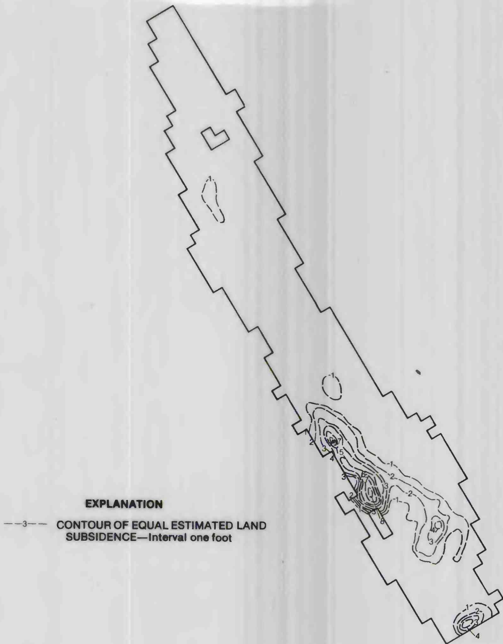
FIGURE 40A.—Estimated land subsidence, 1961-75.
