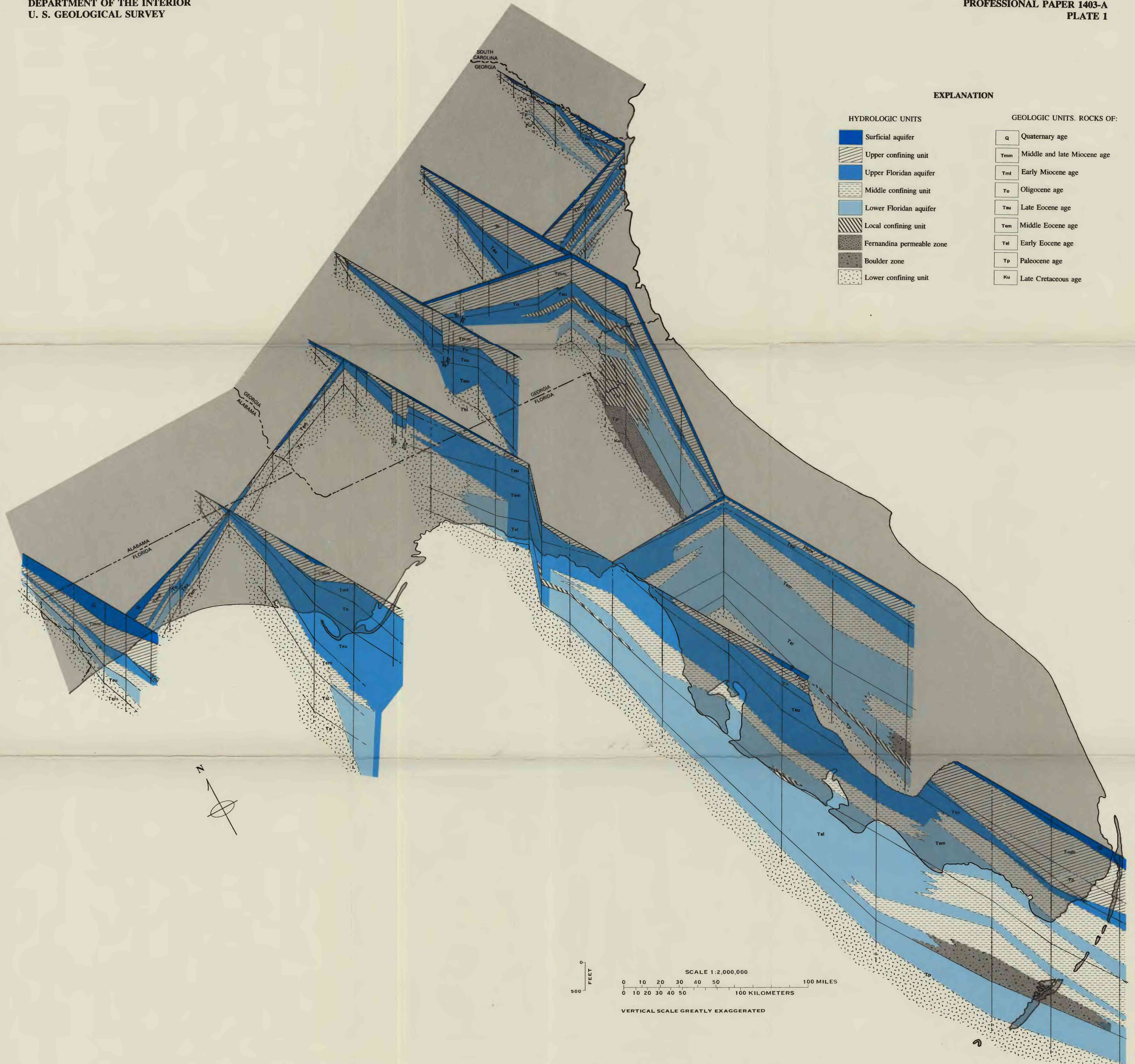
GENERALIZED FENCE DIAGRAM SHOWING RELATION OF GEOLOGIC UNITS TO AQUIFERS AND CONFINING UNITS OF THE FLORIDAN AQUIFER SYSTEM
