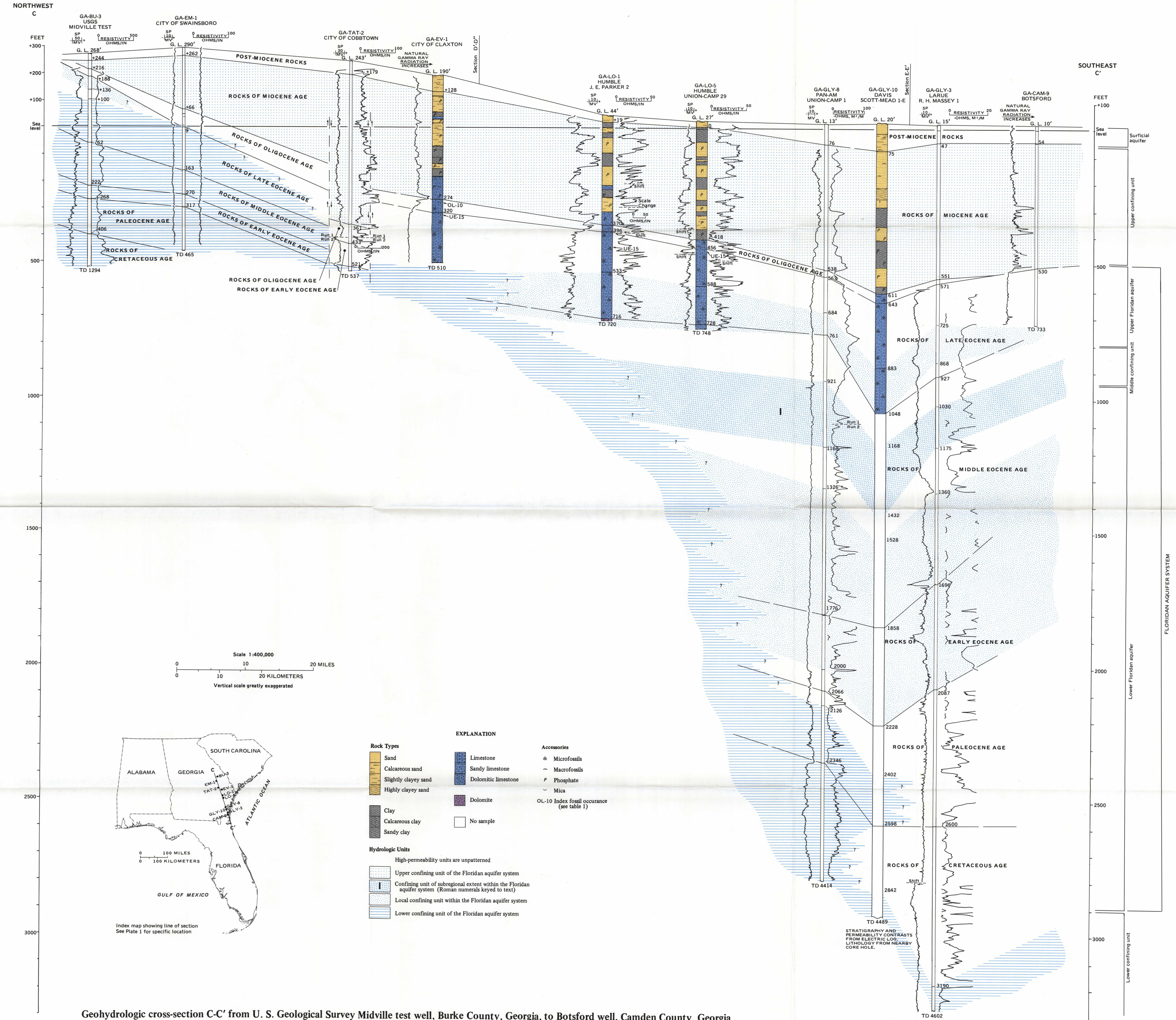
Geohydrologic cross-section C-C' from U. S. Geological Survey Midville test well, Burke County, Georgia, to Botsford well, Camden County, Georgia.
