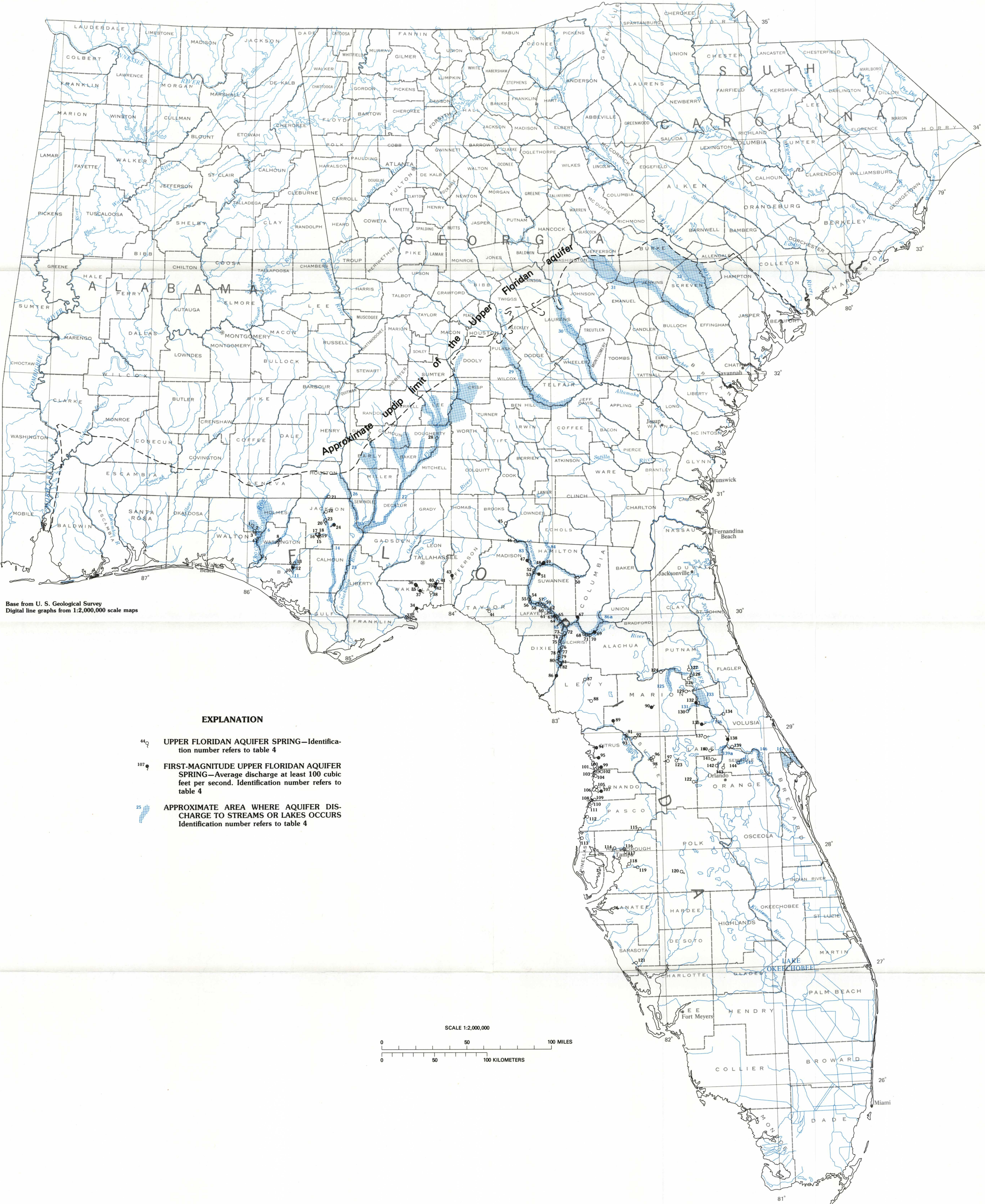
LOCATIONS OF UPPER FLORIDAN AQUIFER SPRINGS AND AREAS OF UPPER FLORIDAN AQUIFER DISCHARGE TO SURFACE-WATER BODIES
