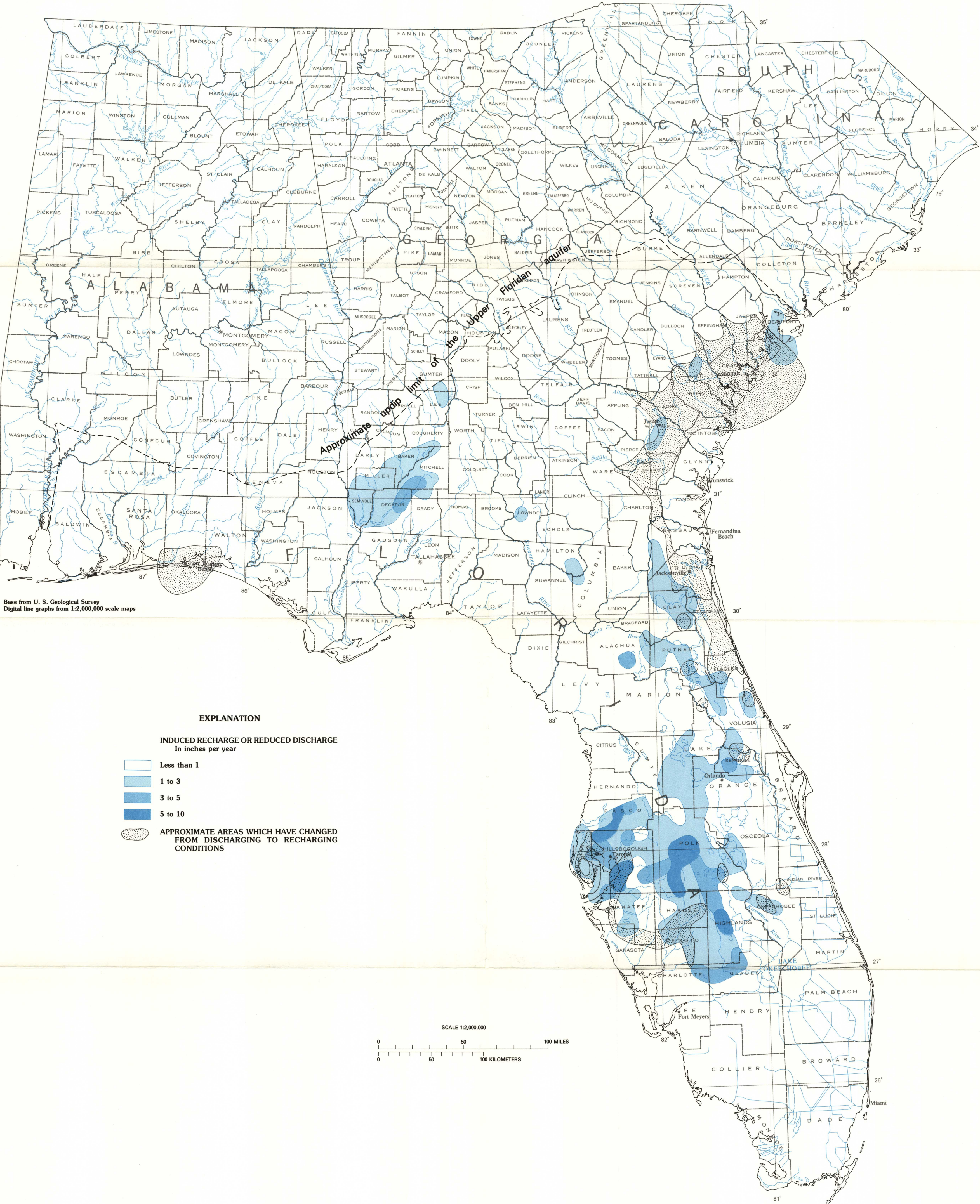
ESTIMATED CHANGES IN RECHARGE TO AND DISCHARGE (AS DIFFUSE UPWARD LEAKAGE) FROM THE UPPER FLORIDAN AQUIFER DUE TO CURRENT (ABOUT 1980) PUMPAGE
