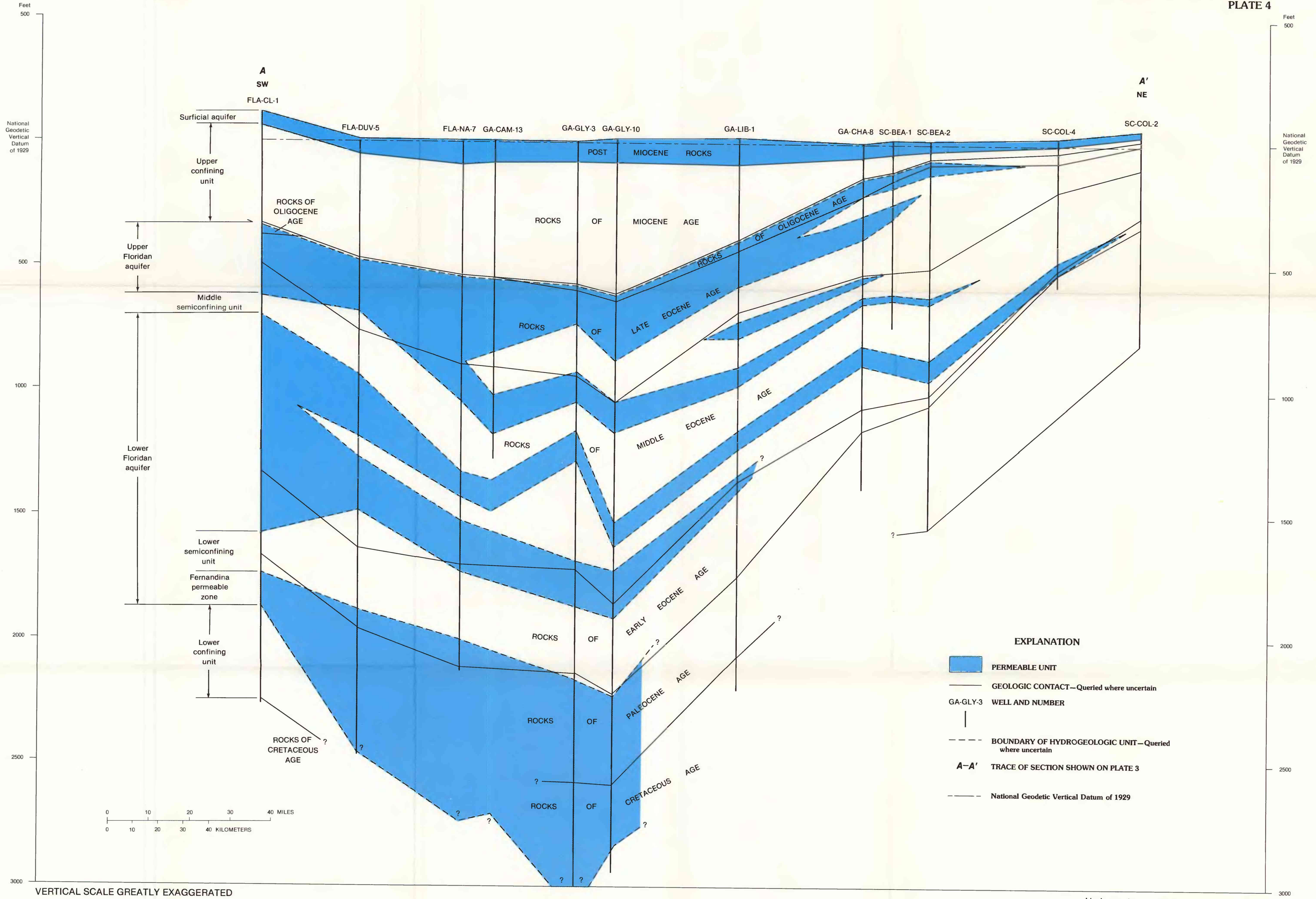
GENERALIZED HYDROGEOLOGIC SECTION SHOWING FLORIDAN AQUIFER SYSTEM ALONG THE ATLANTIC COAST, NORTHEAST FLORIDA TO SOUTHERN SOUTH CAROLINA
