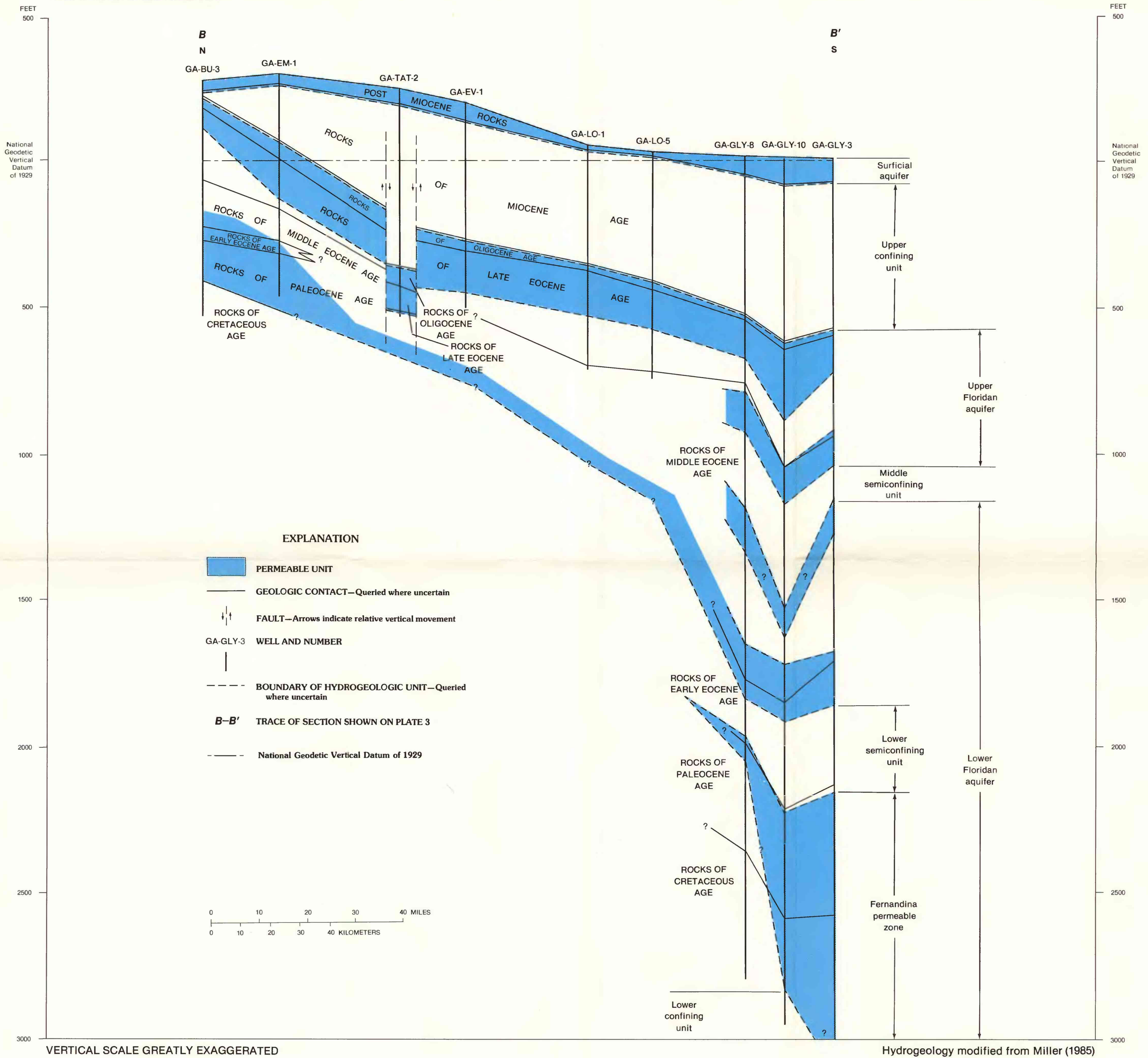
GENERALIZED HYDROGEOLOGIC SECTION SHOWING FLORIDAN AQUIFER SYSTEM APPROXIMATELY ALONG DIP, EAST-CENTRAL TO SOUTHEAST GEORGIA
