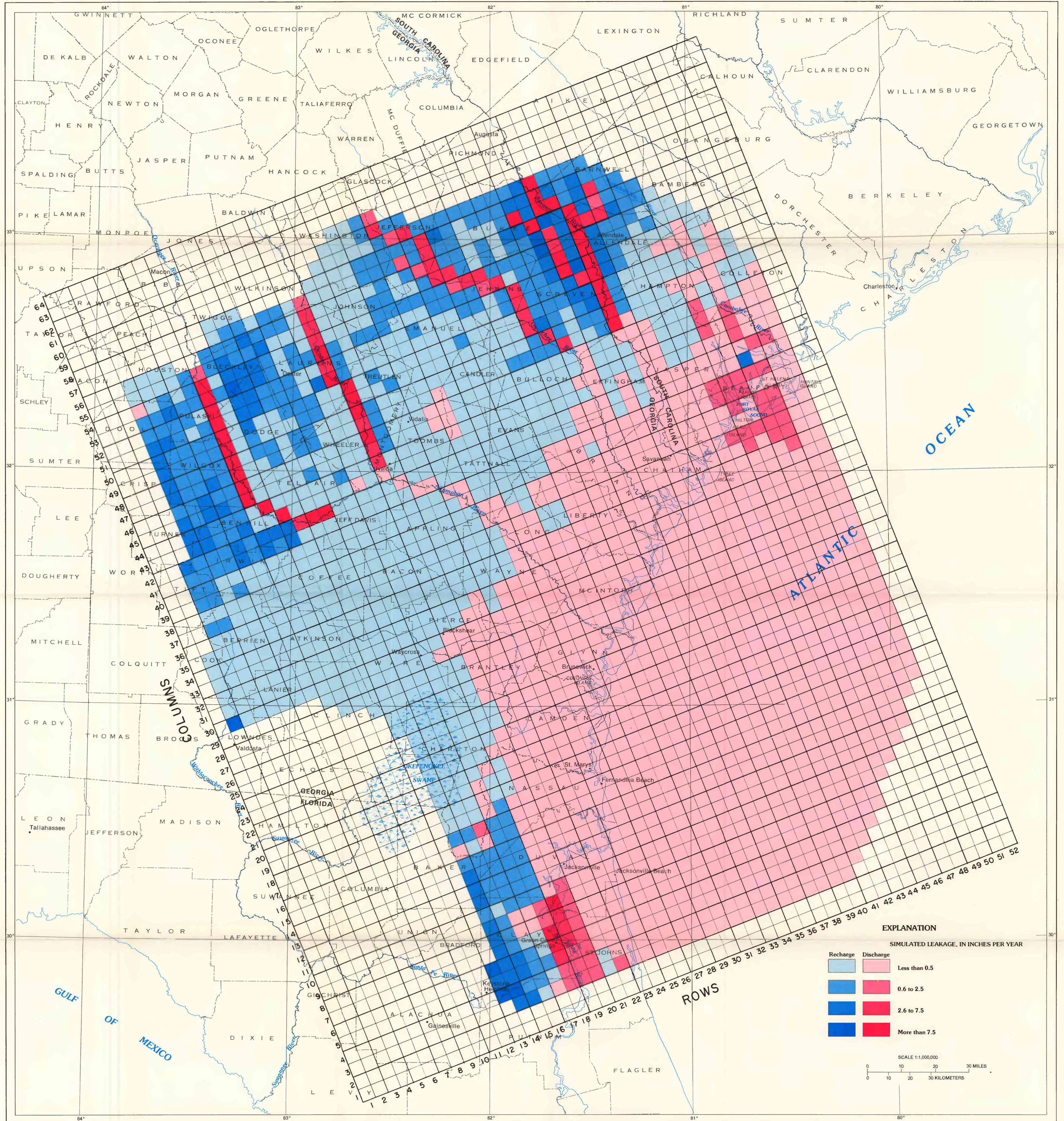
LEAKAGE THROUGH THE UPPER CONFINING UNIT, BASED ON SIMULATION OF THE PREDEVELOPMENT FLOW SYSTEM OF THE FLORIDAN AQUIFER SYSTEM IN SOUTHEAST GEORGIA AND ADJACENT PARTS OF FLORIDA AND SOUTH CAROLINA
