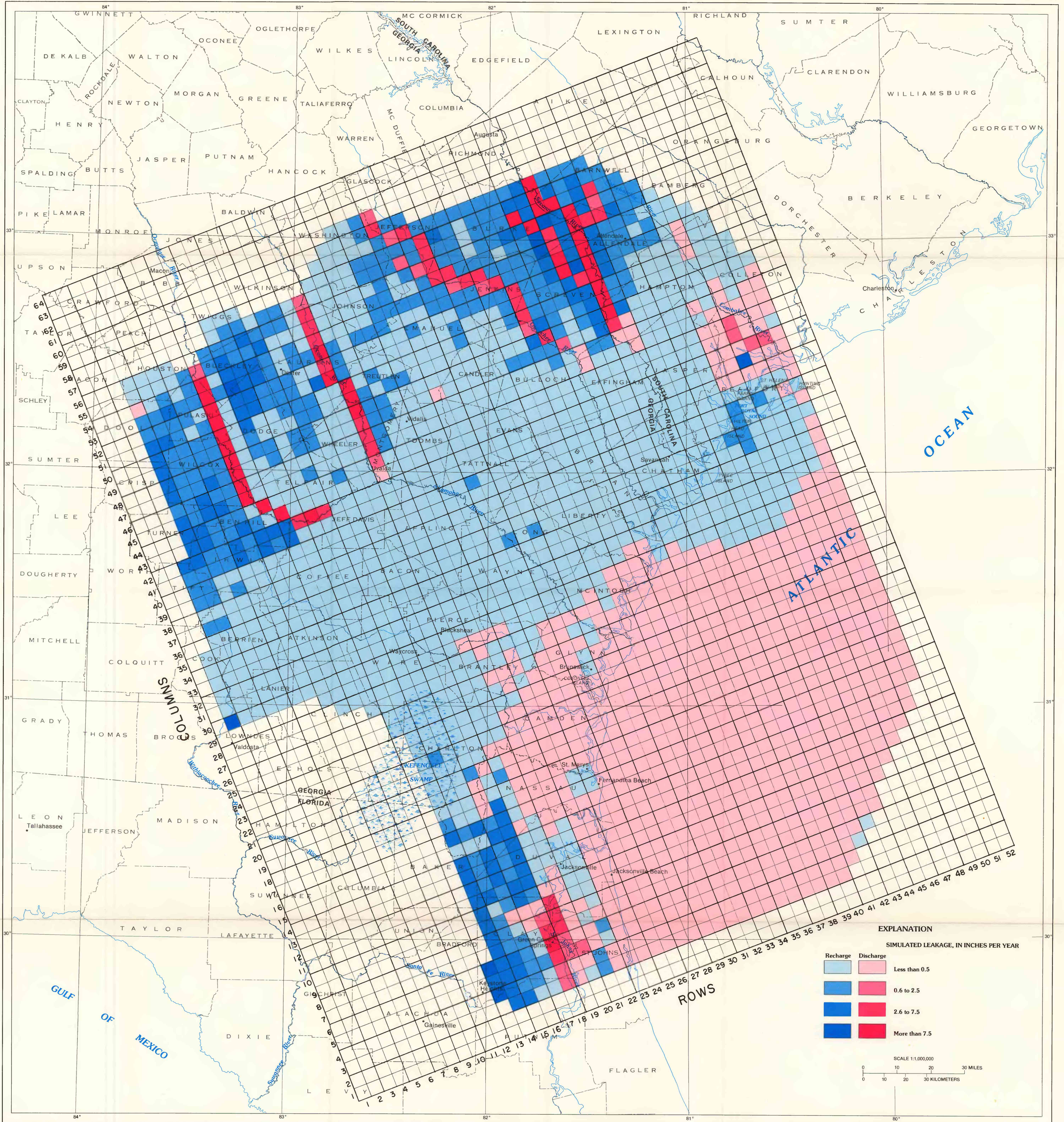
LEAKAGE THROUGH THE UPPER CONFINING UNIT, BASED ON SIMULATION OF THE PRESENT-DAY (1980) FLOW SYSTEM OF THE FLORIDAN AQUIFER SYSTEM IN SOUTHEAST GEORGIA AND ADJACENT PARTS OF FLORIDA AND SOUTH CAROLINA
