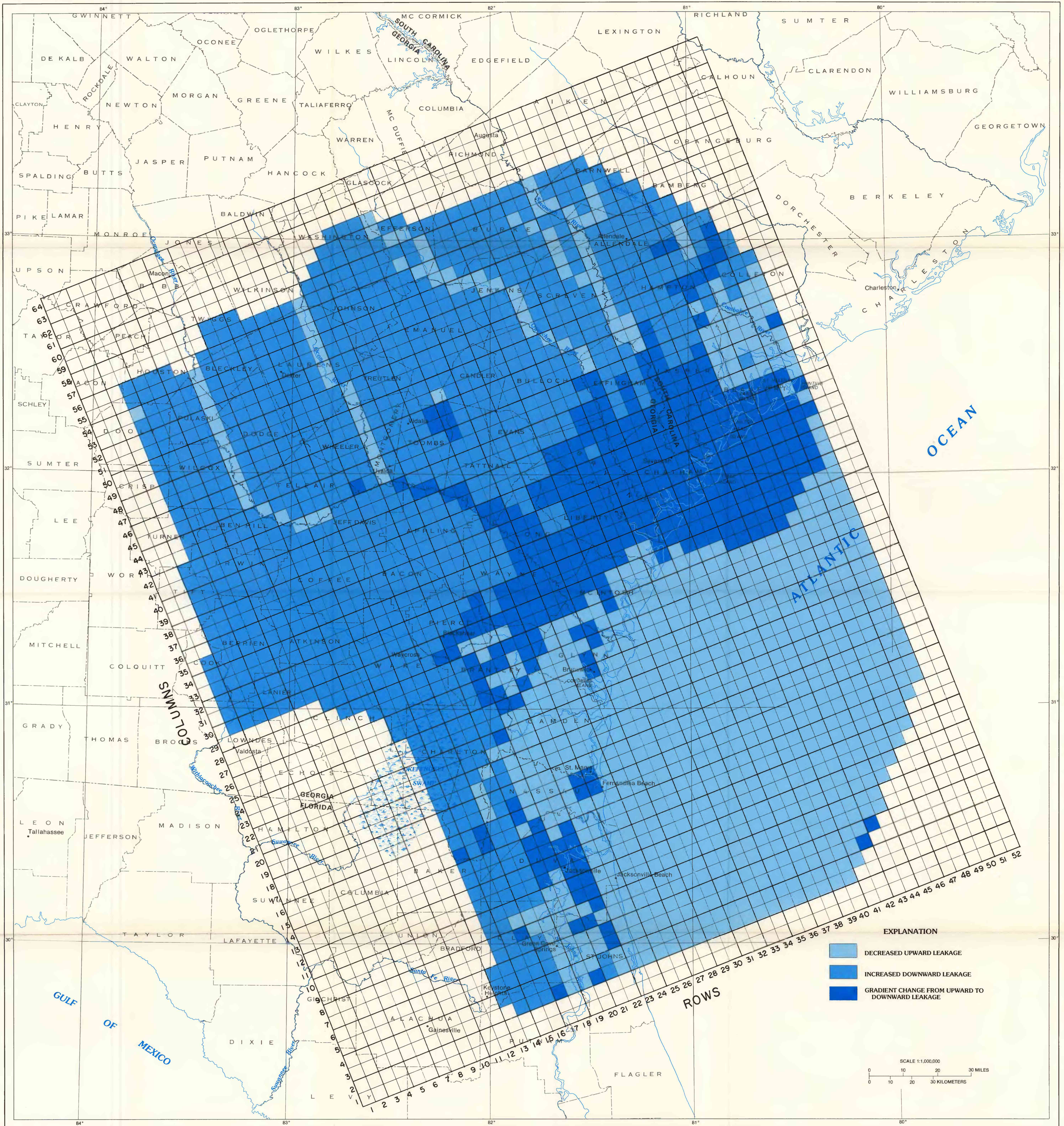
COMPARISON OF SIMULATED LEAKAGE THROUGH THE UPPER CONFINING UNIT OF THE FLORIDAN AQUIFER SYSTEM BETWEEN PREDEVELOPMENT (1880) AND PRESENT-DAY (1980) CONDITIONS IN SOUTHEAST GEORGIA AND ADJACENT PARTS OF FLORIDA AND SOUTH CAROLINA
