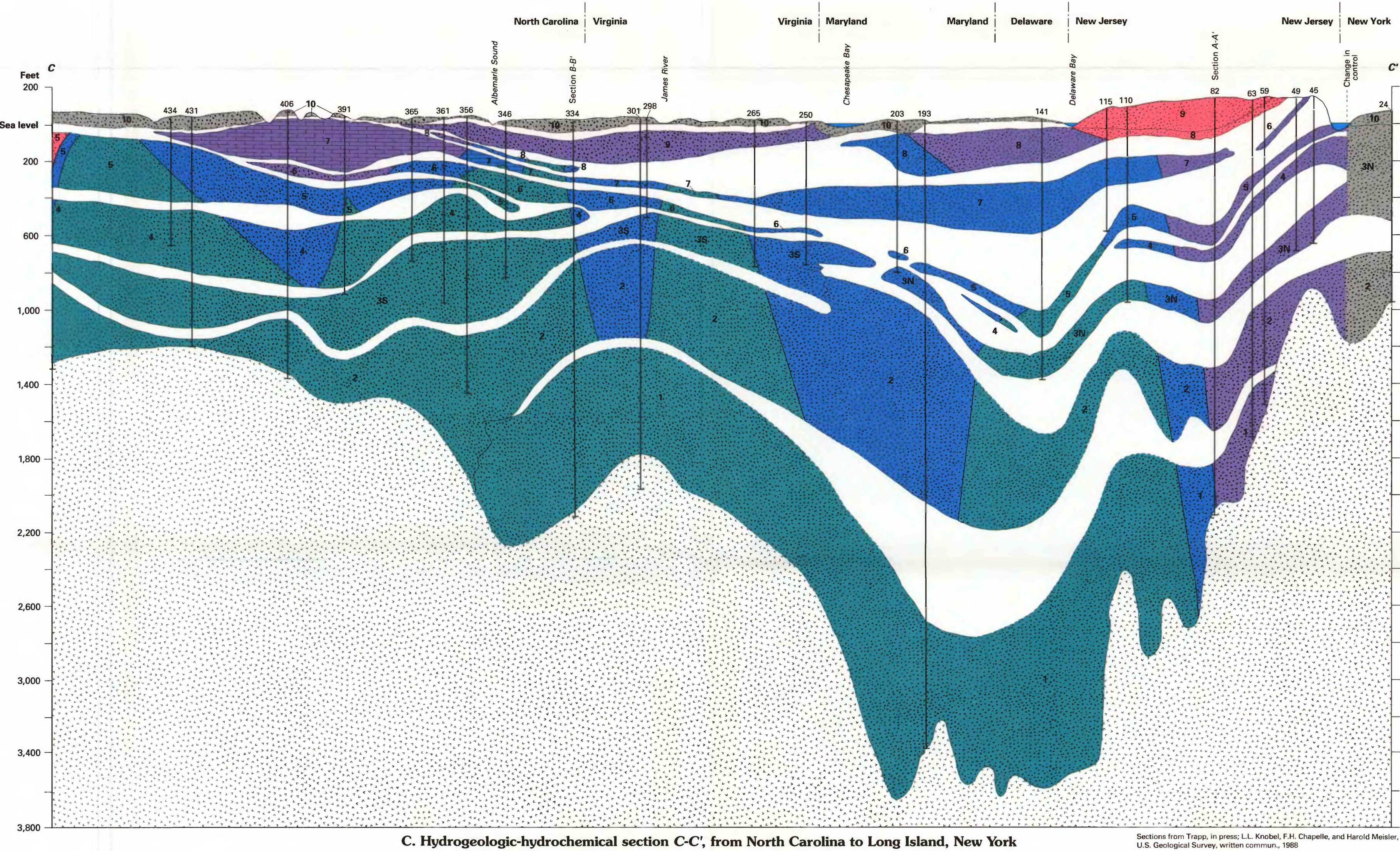
Hydrogeologic-hydrochemical sections (A) A-A' in New Jersey, (B) B-B' in North Carolina, and (C) C-C' from North Carolina to Long Island, New York
