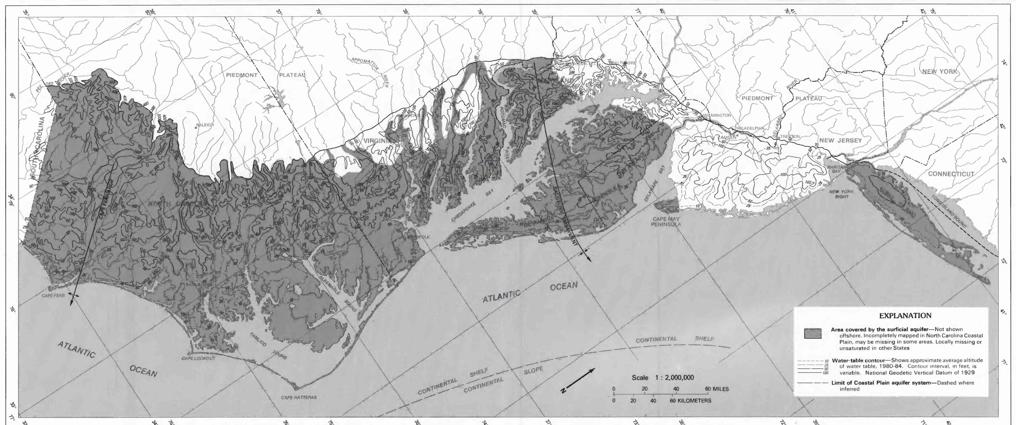
B. Approximate average altitude of the water table for 1980-1984 and extent of the surficial aquifer
