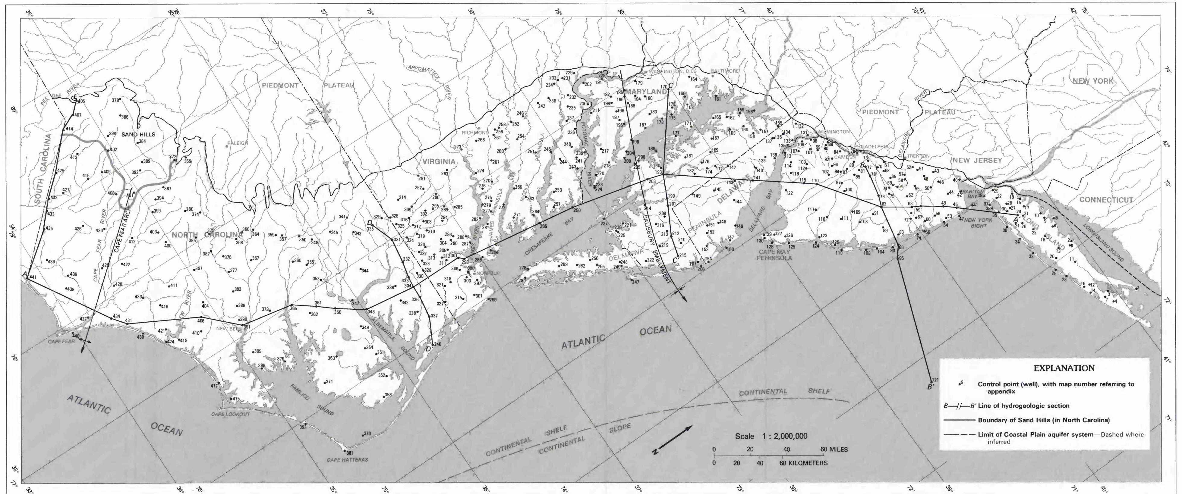
A. Locations of wells and hydrogeologic sections in the northern Atlantic Coastal Plain
