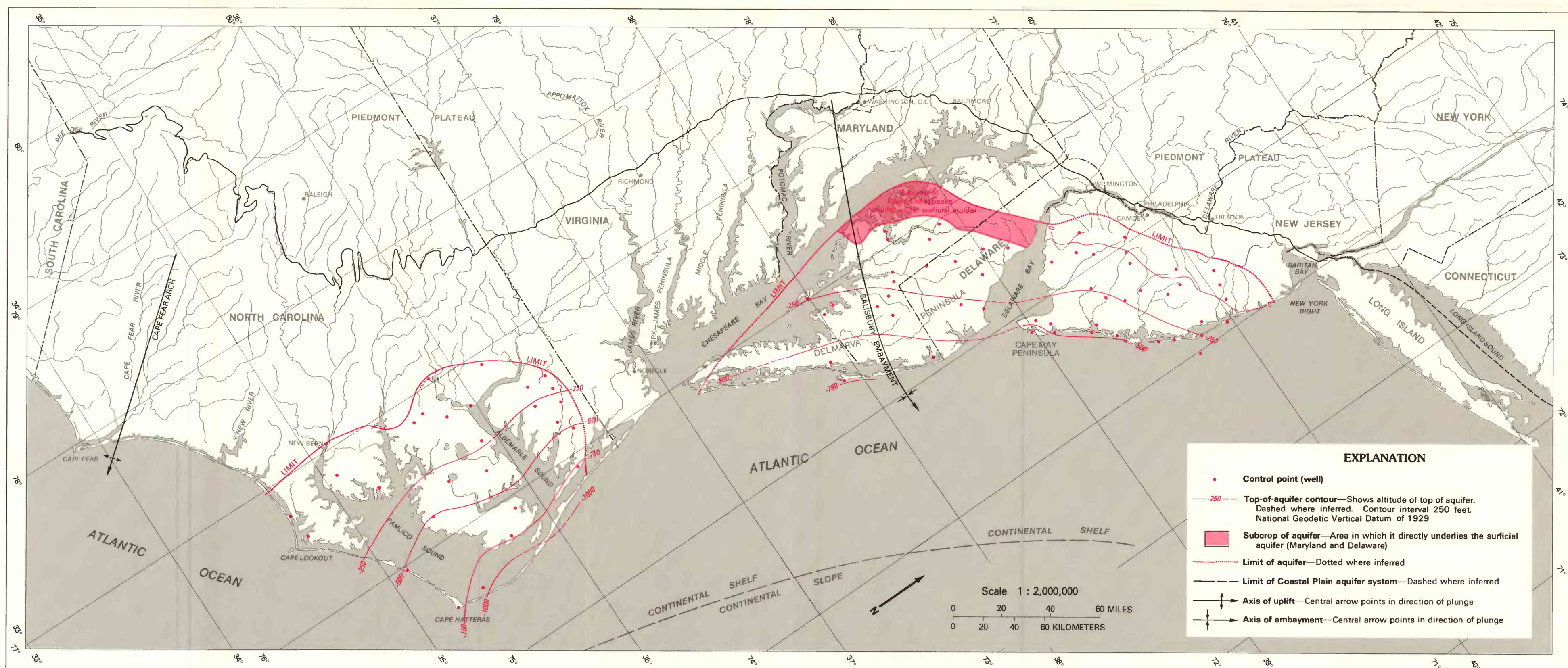
B. Altitude of the top of the lower Chesapeake aquifer
