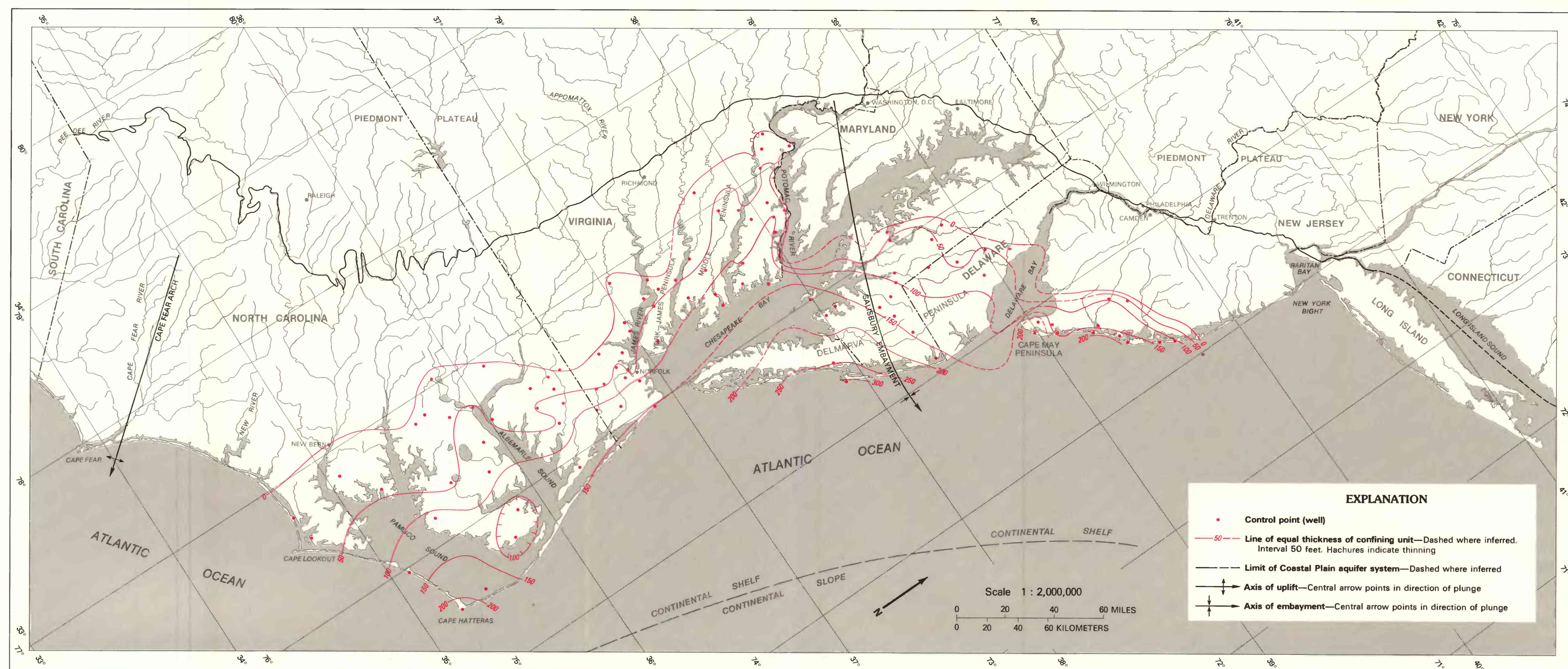
A. Thickness of the confining unit overlying the lower Chesapeake aquifer
