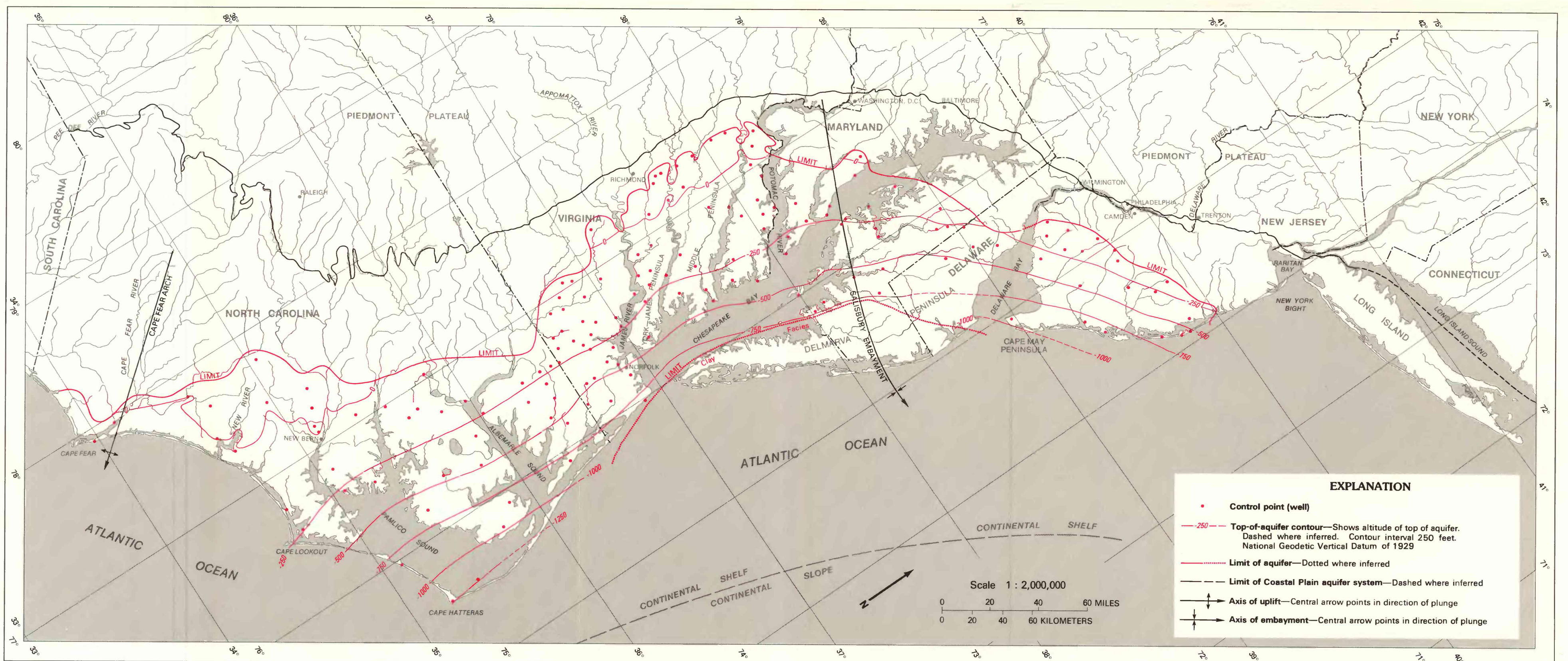
B. Altitude of the top of the Castle Hayne-Piney Point aquifer
