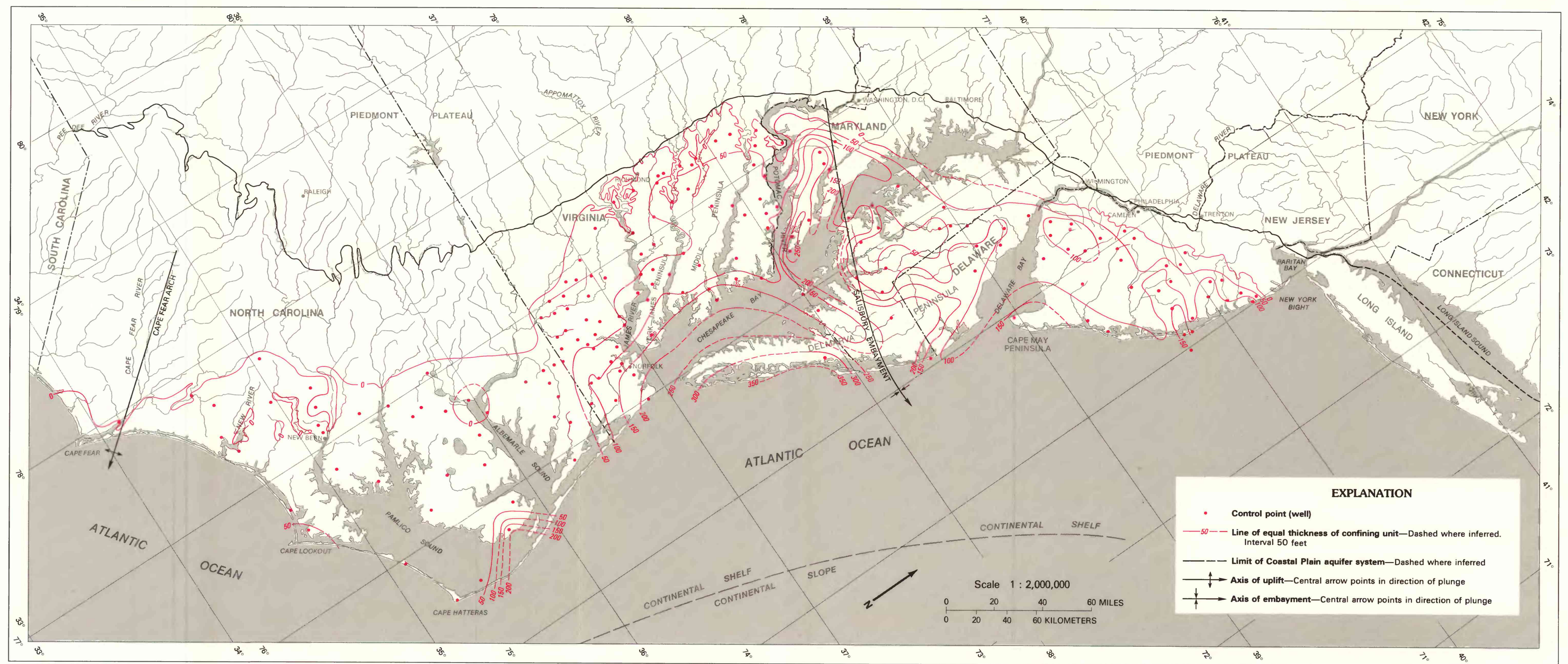
A. Thickness of the confining unit overlying the Castle Hayne-Piney Point aquifer
