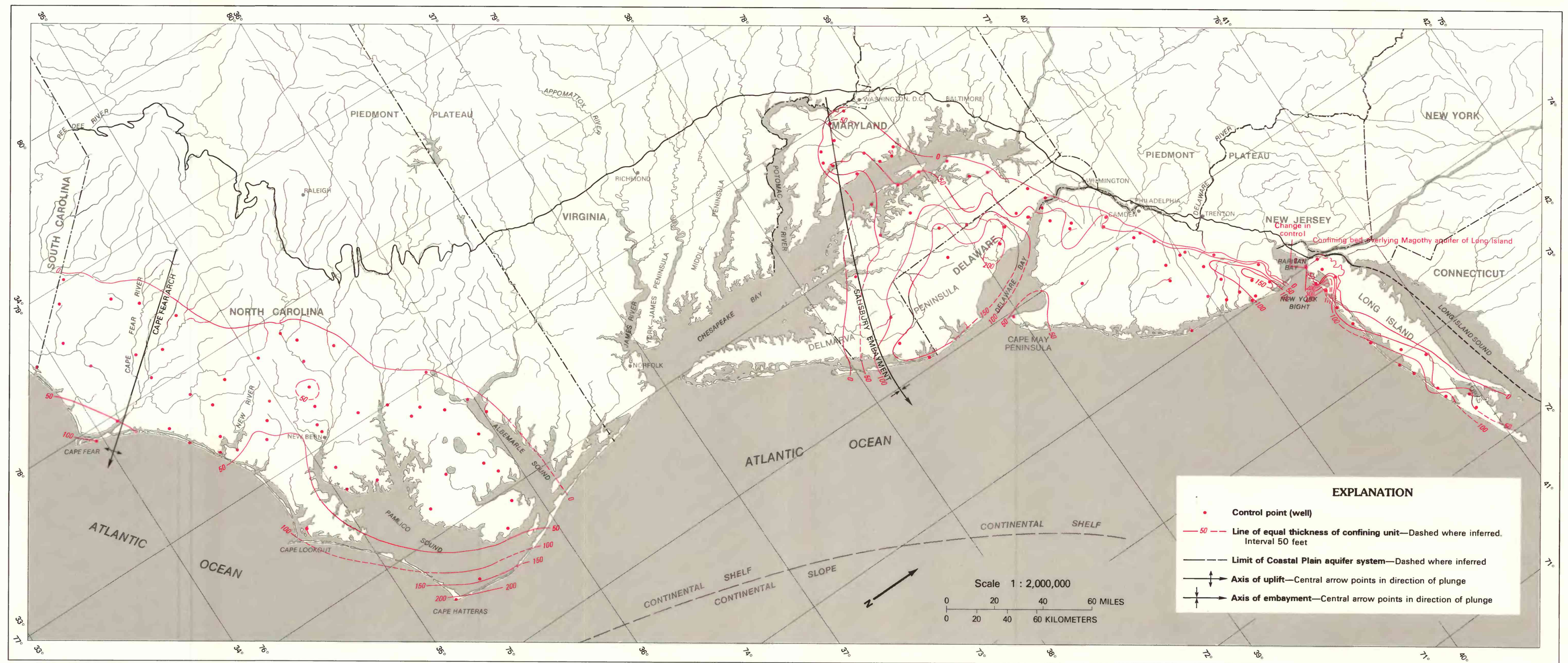
A. Thickness of the confining unit overlying the Peedee-Severn aquifer and the Magothy aquifer of Long Island
