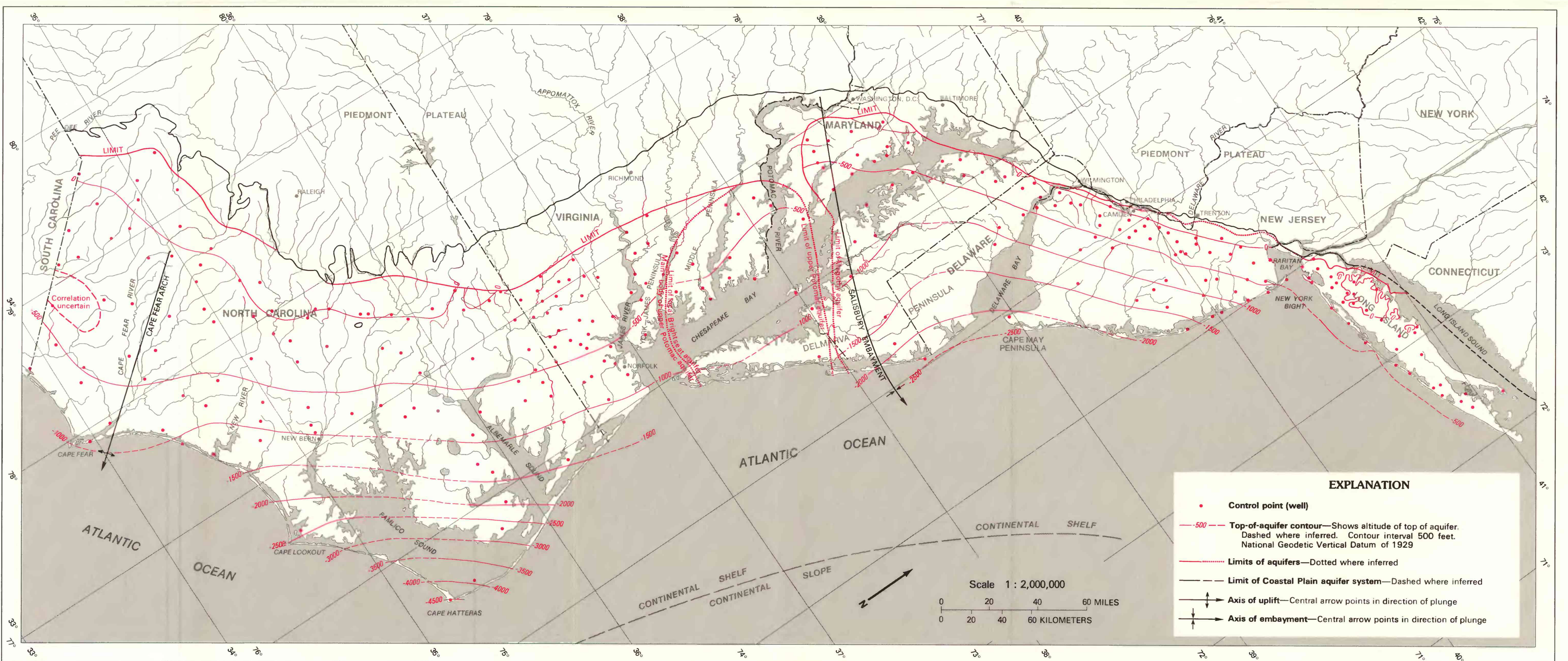
B. Altitude of the top of the upper Potomac and Magothy aquifers
