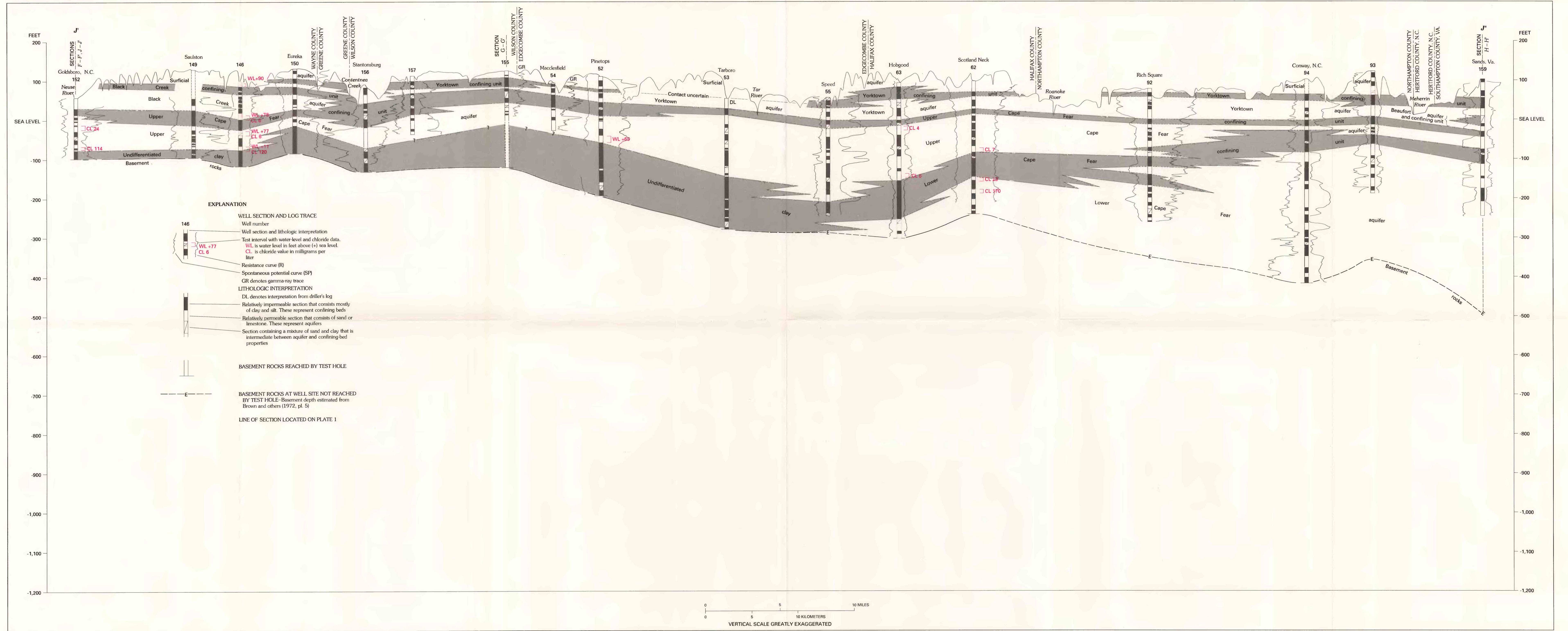
HYDROGEOLOGIC SECTION J' - J'' FROM GOLDSBORO, WAYNE COUNTY, NORTH CAROLINA, TO SANDS, SOUTHAMPTON COUNTY, VIRGINIA
