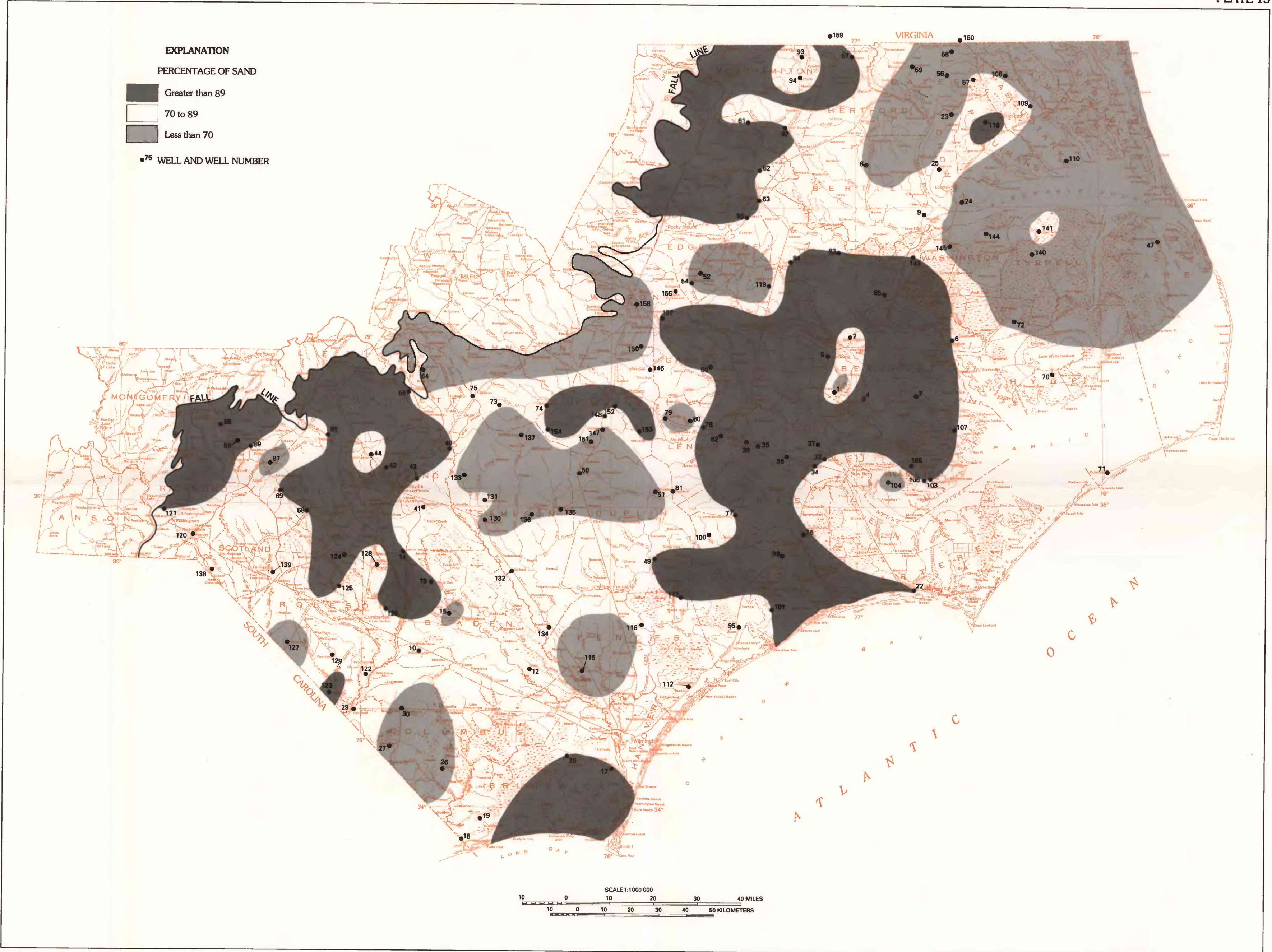
MAP SHOWING PERCENTAGE OF SAND IN THE SURFICIAL AQUIFER OF THE NORTH CAROLINA COASTAL PLAIN
