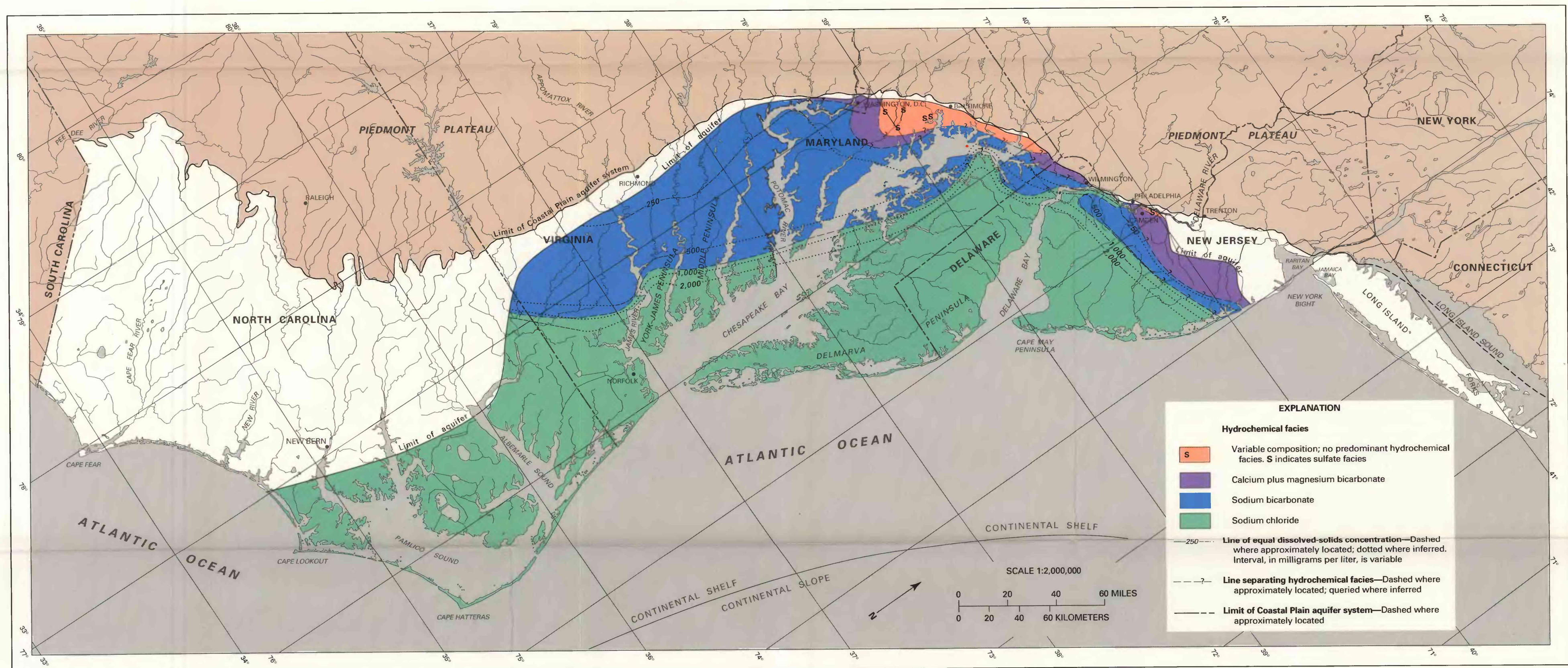
B. Areal extent, hydrochemical facies, and dissolved-solids concentrations of the lower Potomac aquifer
