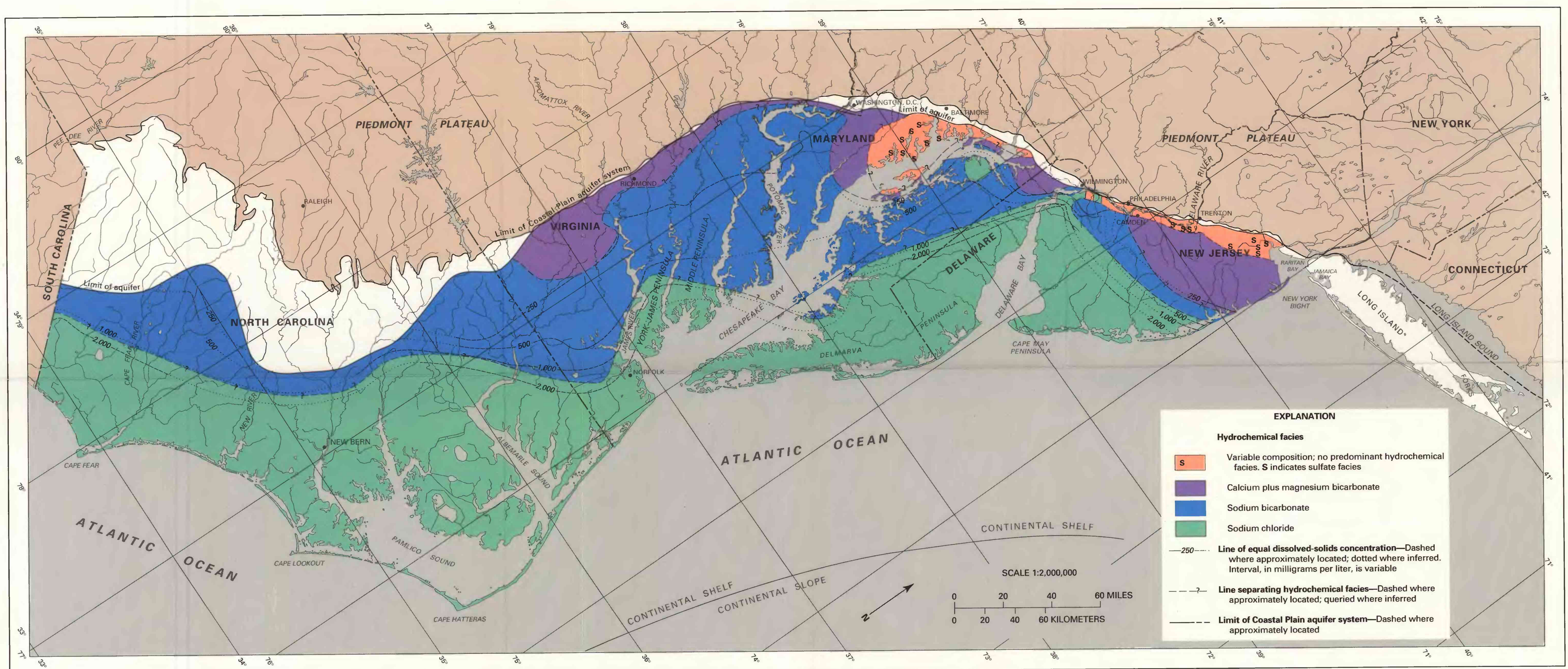
A. Areal extent, hydrochemical facies, and dissolved-solids concentrations of the middle Potomac aquifer
