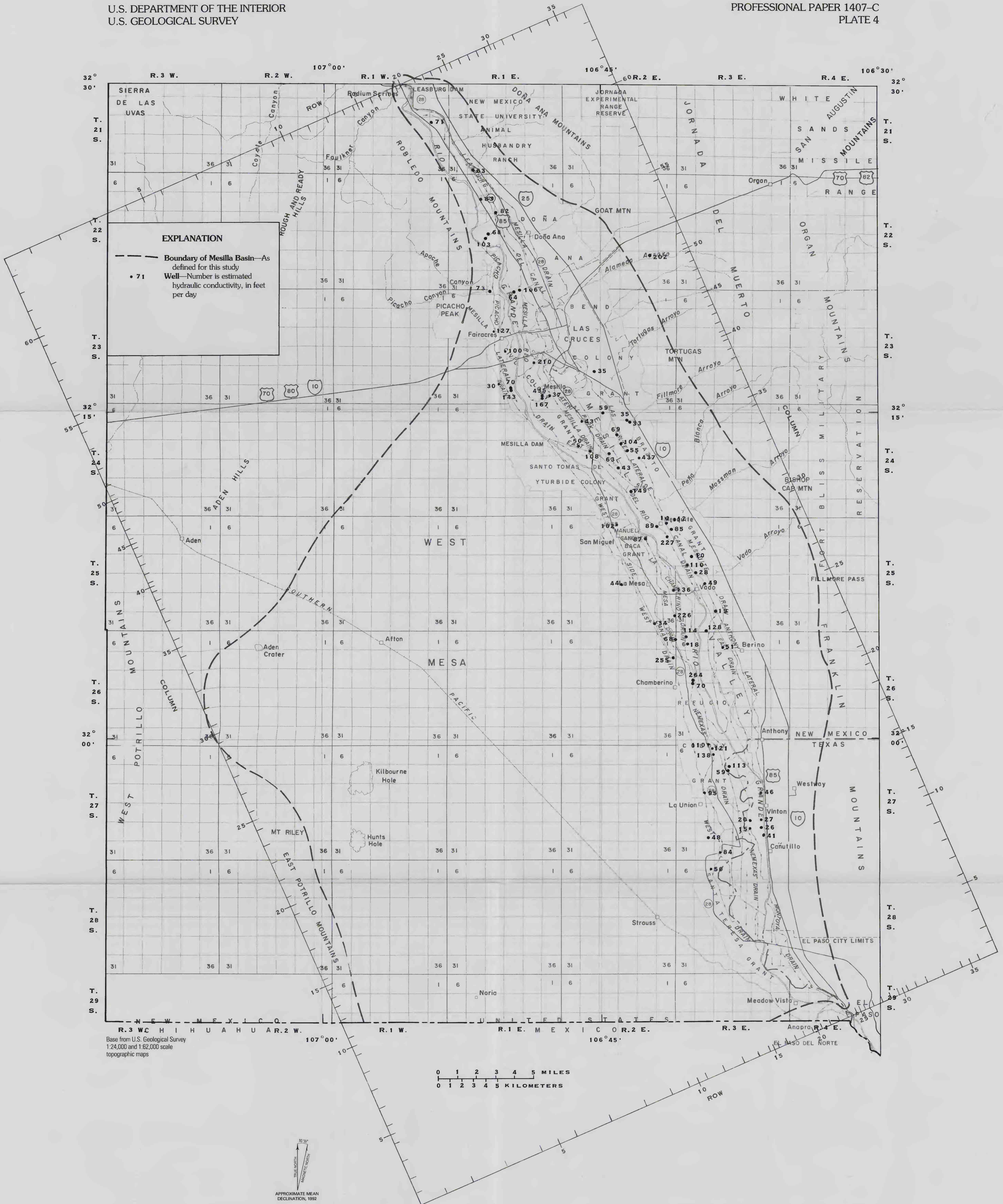
MAP SHOWING ESTIMATED HYDRAULIC CONDUCTIVITY OF THE SHALLOW PART OF THE AQUIFER (FLOOD-PLAIN ALLUVIUM AND UPPER PART OF THE SANTA FE GROUP), MESILLA VALLEY, NEW MEXICO AND TEXAS
