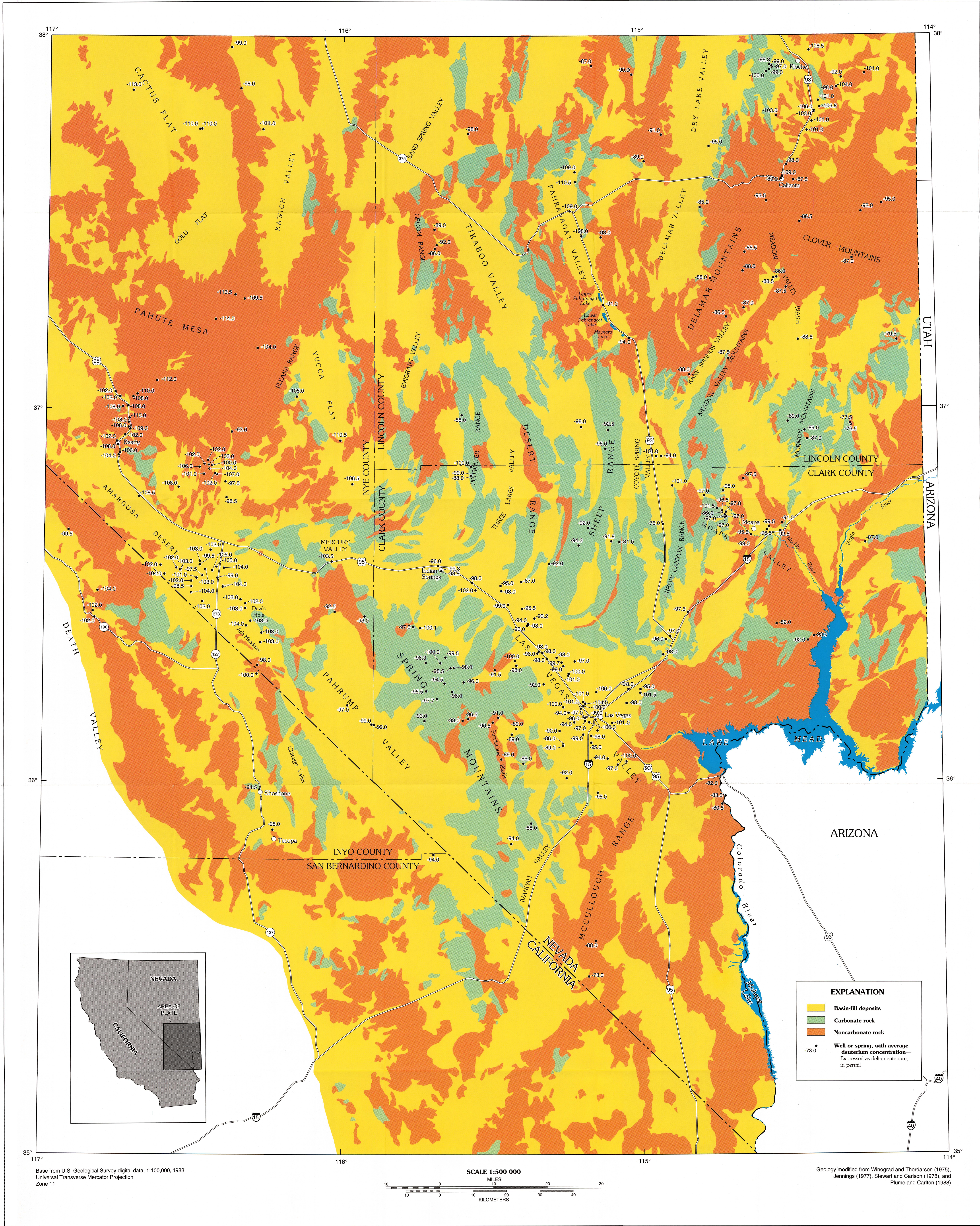
MAP SHOWING AVERAGE DEUTERIUM COMPOSITION FOR WELLS AND SPRINGS IN SOUTHERN NEVADA AND SOUTHEASTERN CALIFORNIA
