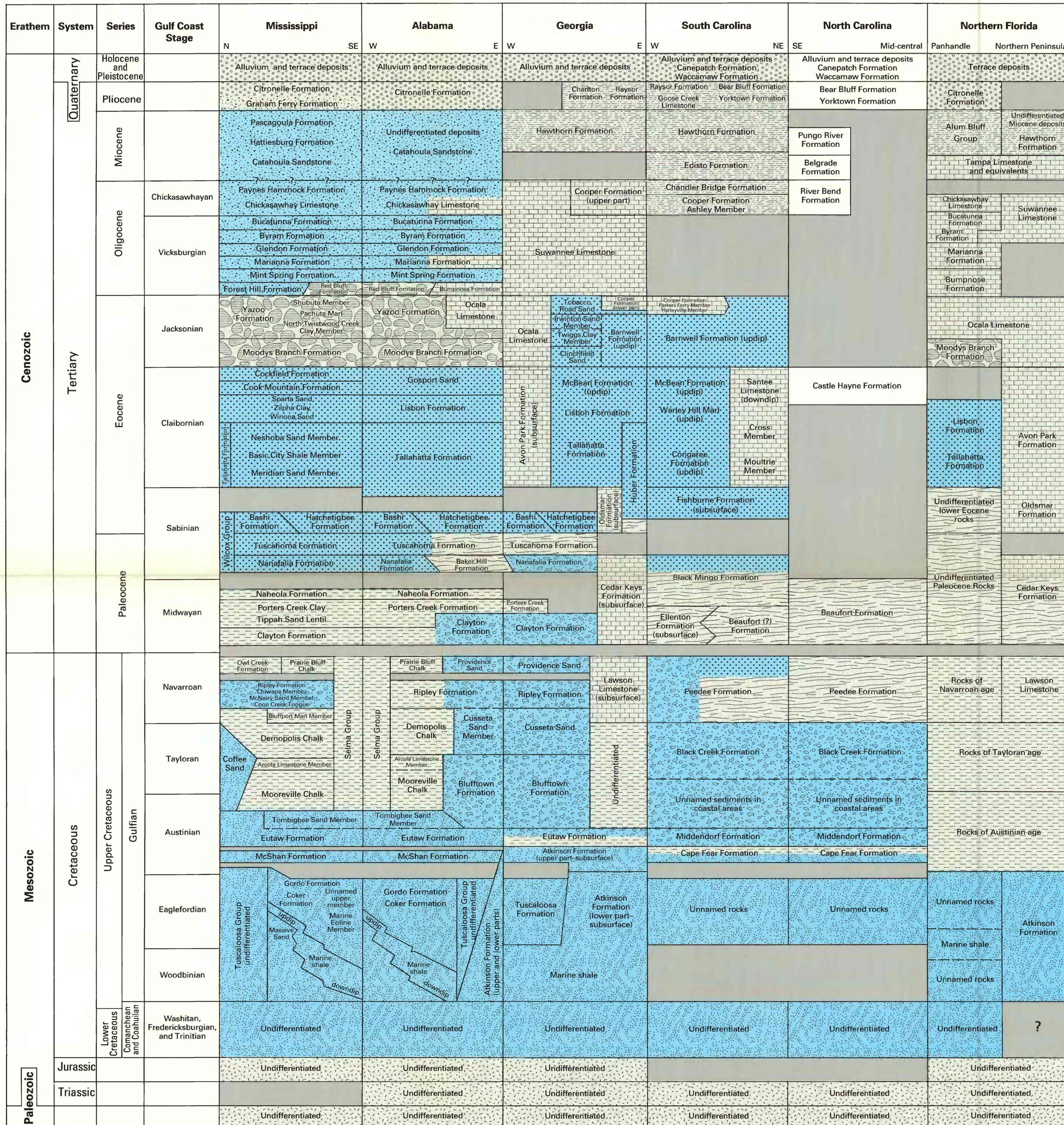
GENERALIZED CORRELATION CHART SHOWING TIME-STRATIGRAPHIC, ROCK-STRATIGRAPHIC, AND REGIONAL HYDROGEOLOGIC UNITS IN THE SOUTHEASTERN COASTAL PLAIN
