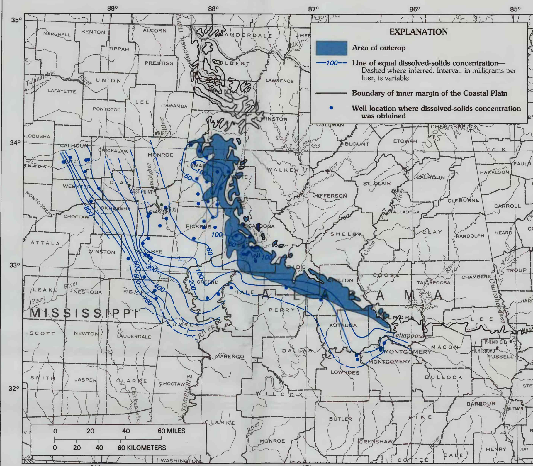
Dissolved solids in the lower water-bearing zone of the Black Warrior River aquifer
