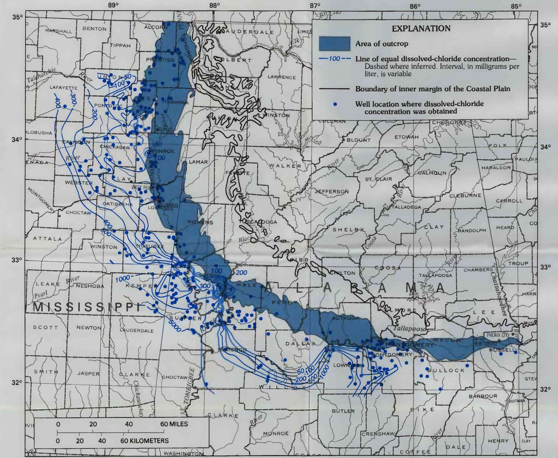
Dissolved chloride in the upper water-bearing zone of the Black Warrior River aquifer
