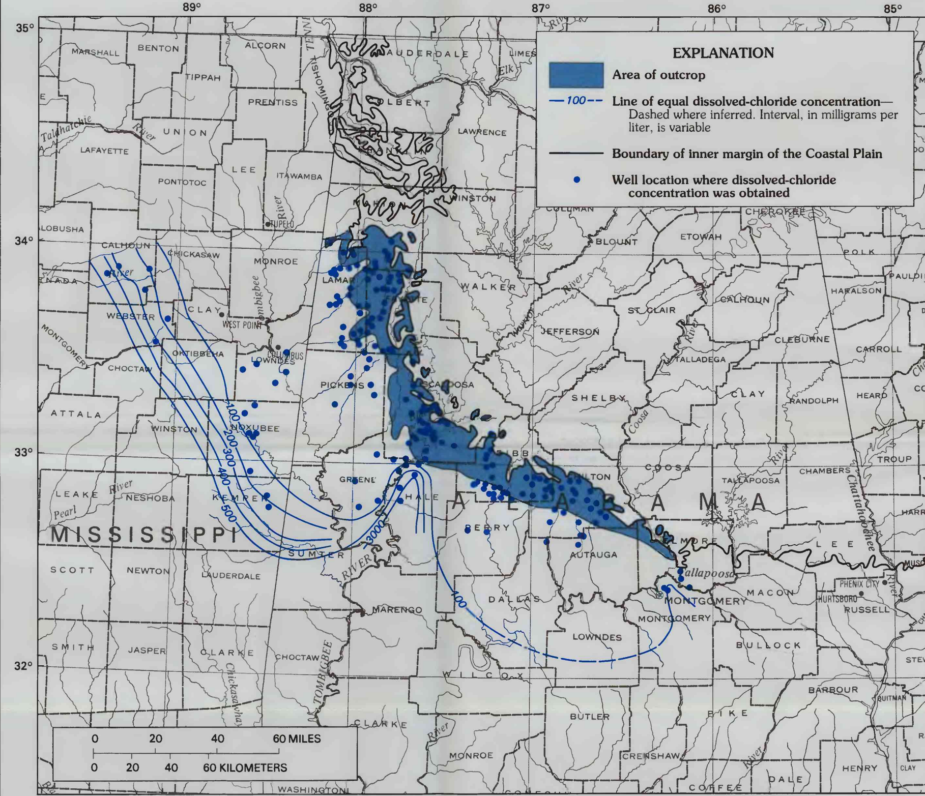
Dissolved chloride in the lower water-bearing zone of the Black Warrior River aquifer
