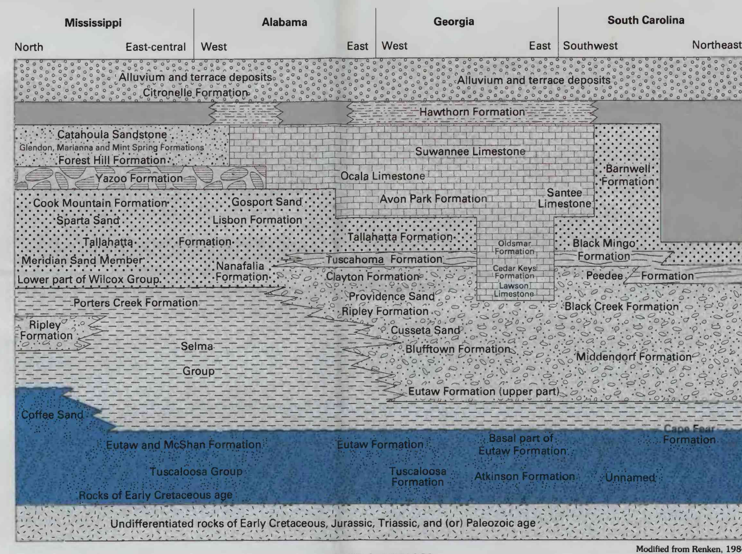
Schematic diagram of regional hydrogeologic units and selected rock-stratigraphic units in the Southeastern Coastal Plain
