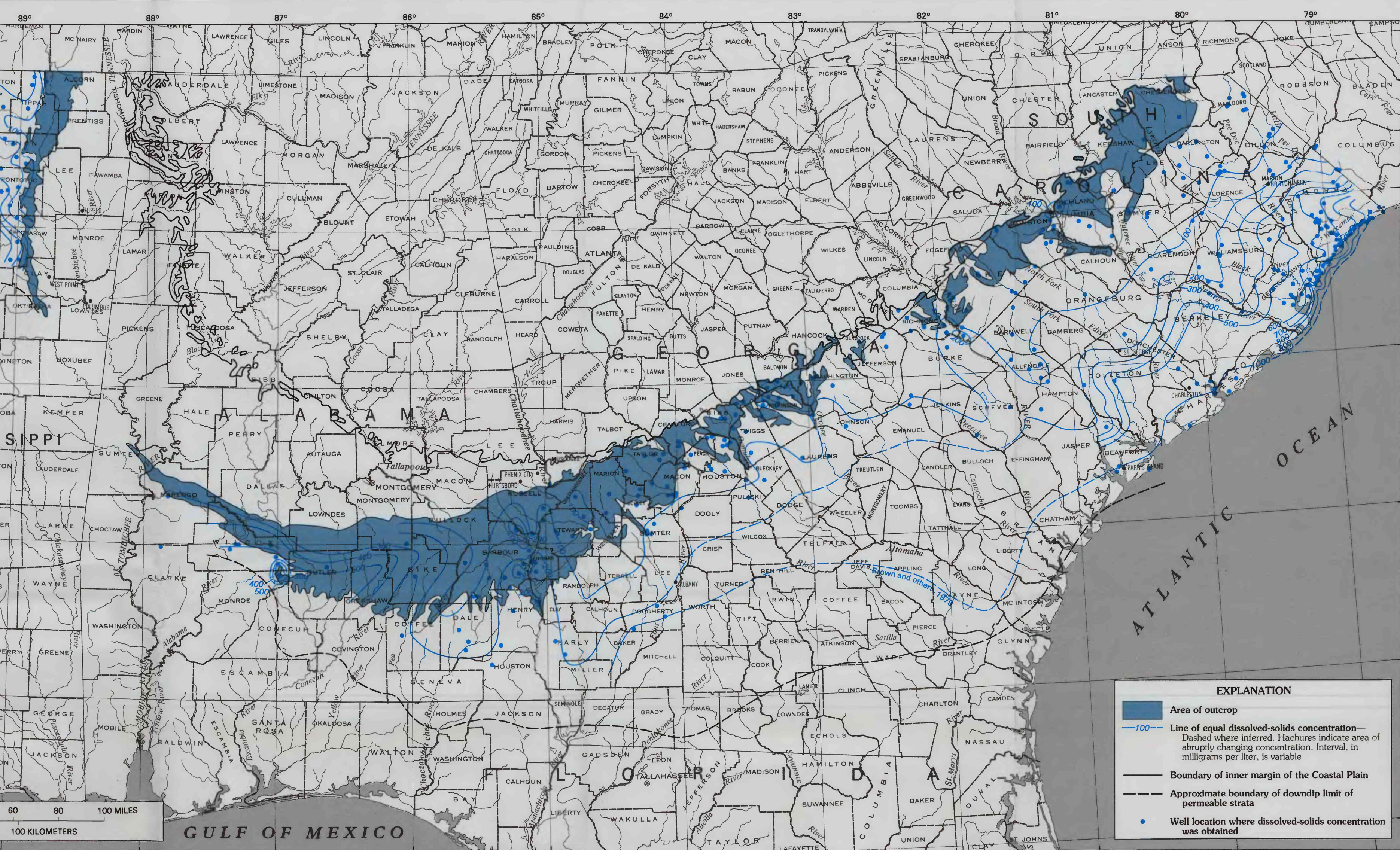
Dissolved solids in the Chattahoochee River aquifer
