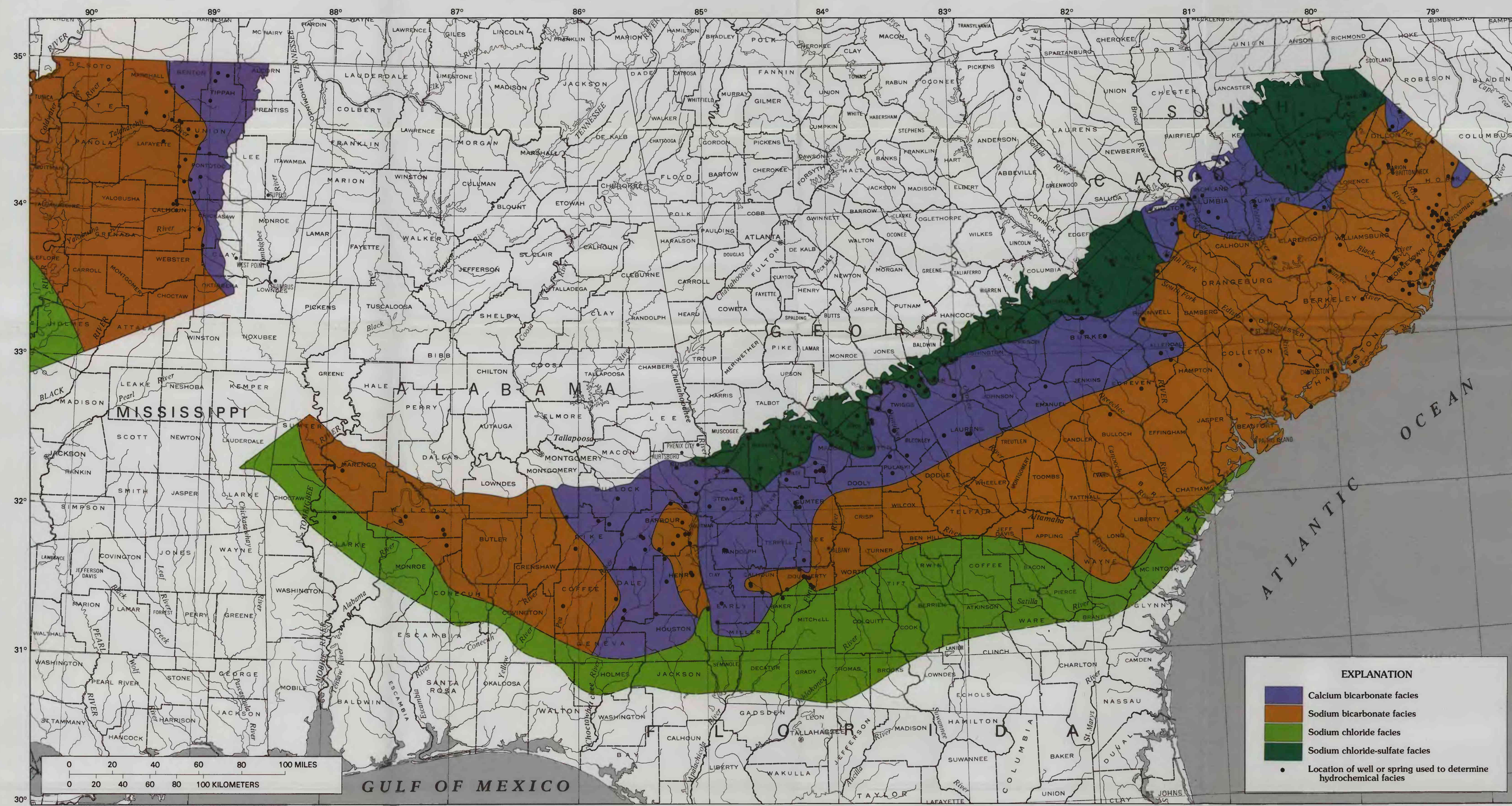
Hydrochemical facies in the Chattahoochee River aquifer
