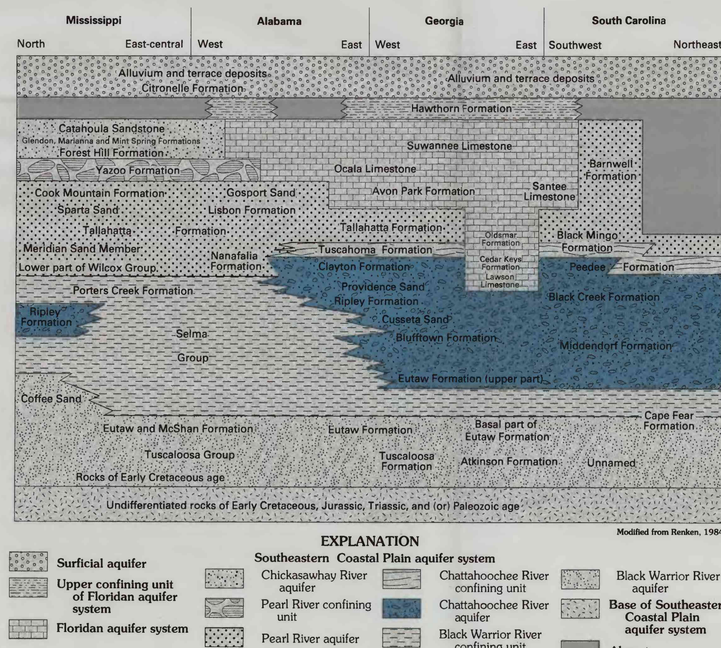
Schematic diagram of regional hydrogeologic units and selected rock-stratigraphic units in the Southeastern Coastal Plain
