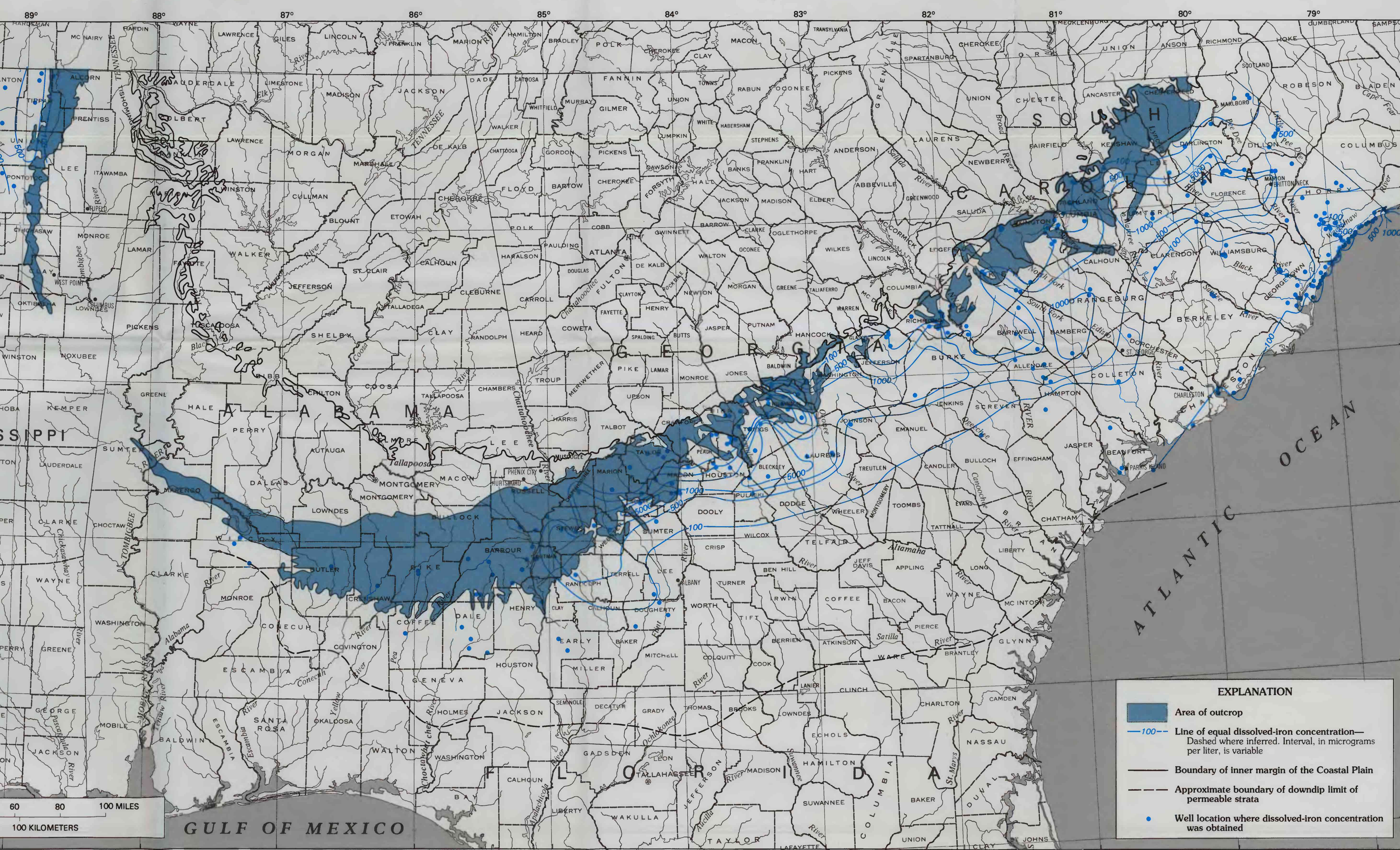
Dissolved iron in the Chattahoochee River aquifer
