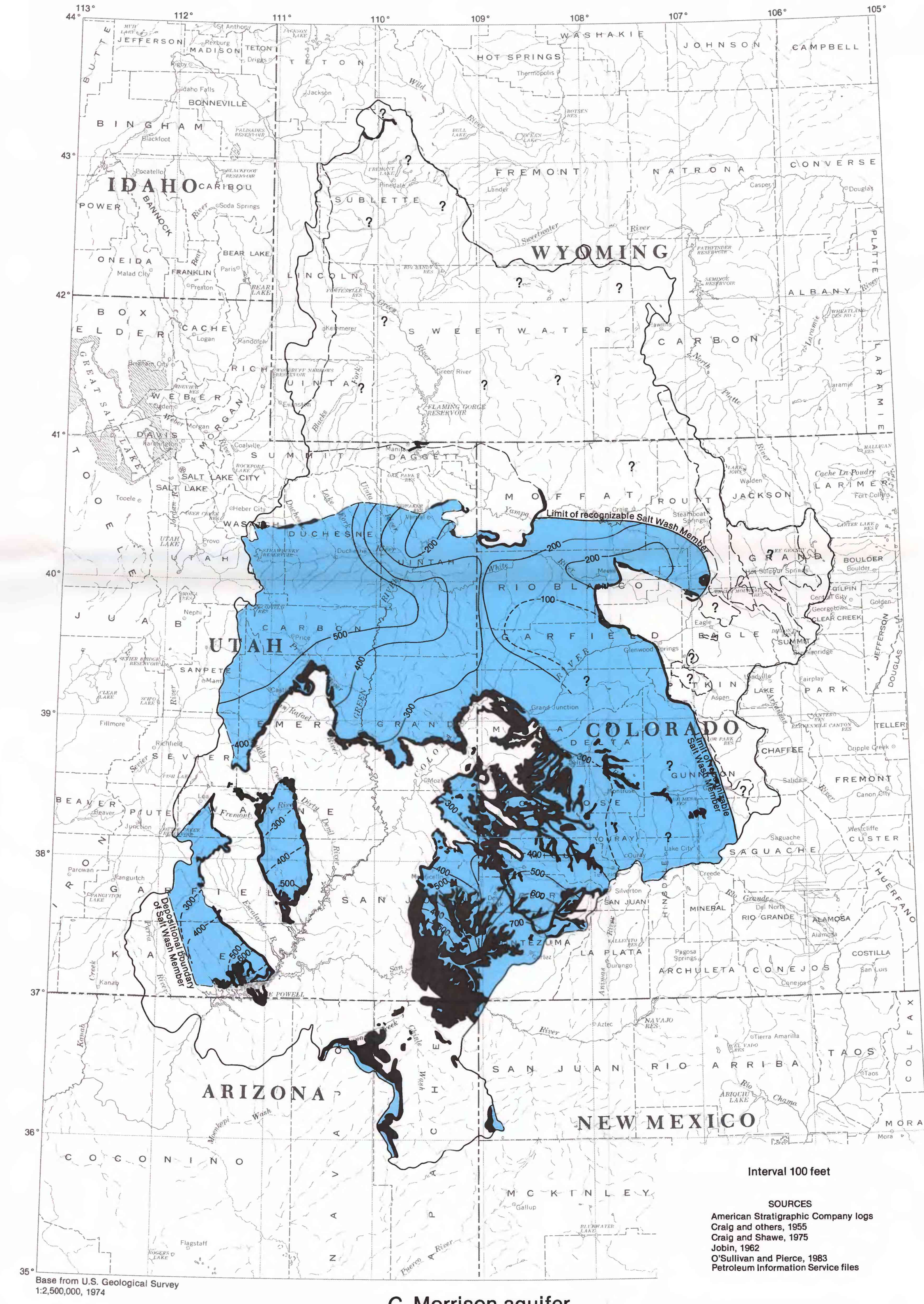
C. Morrison aquifer
