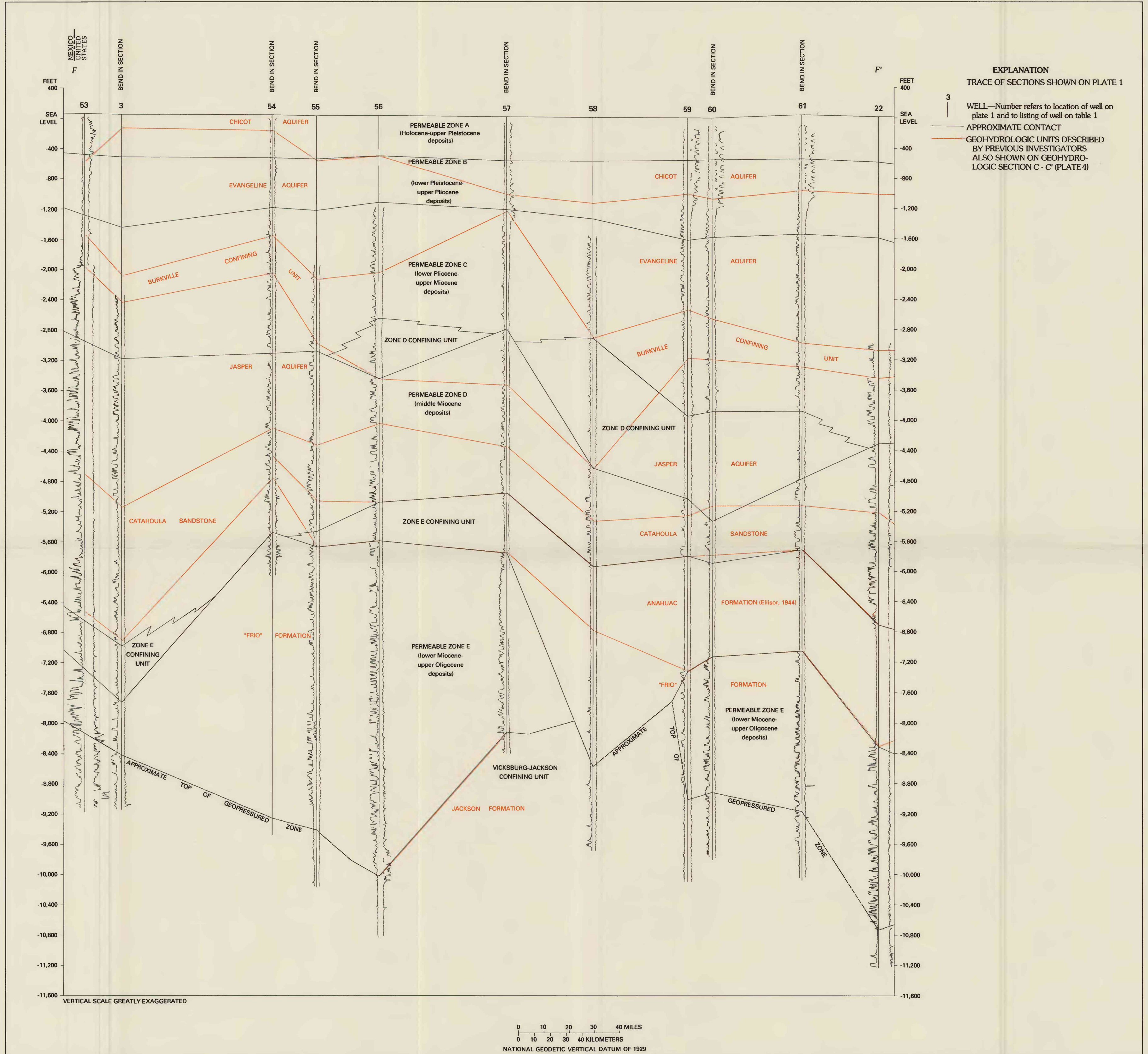
GEOHYDROLOGIC SECTION F - F', COASTAL LOWLANDS AQUIFER SYSTEM, SOUTH-CENTRAL UNITED STATES
