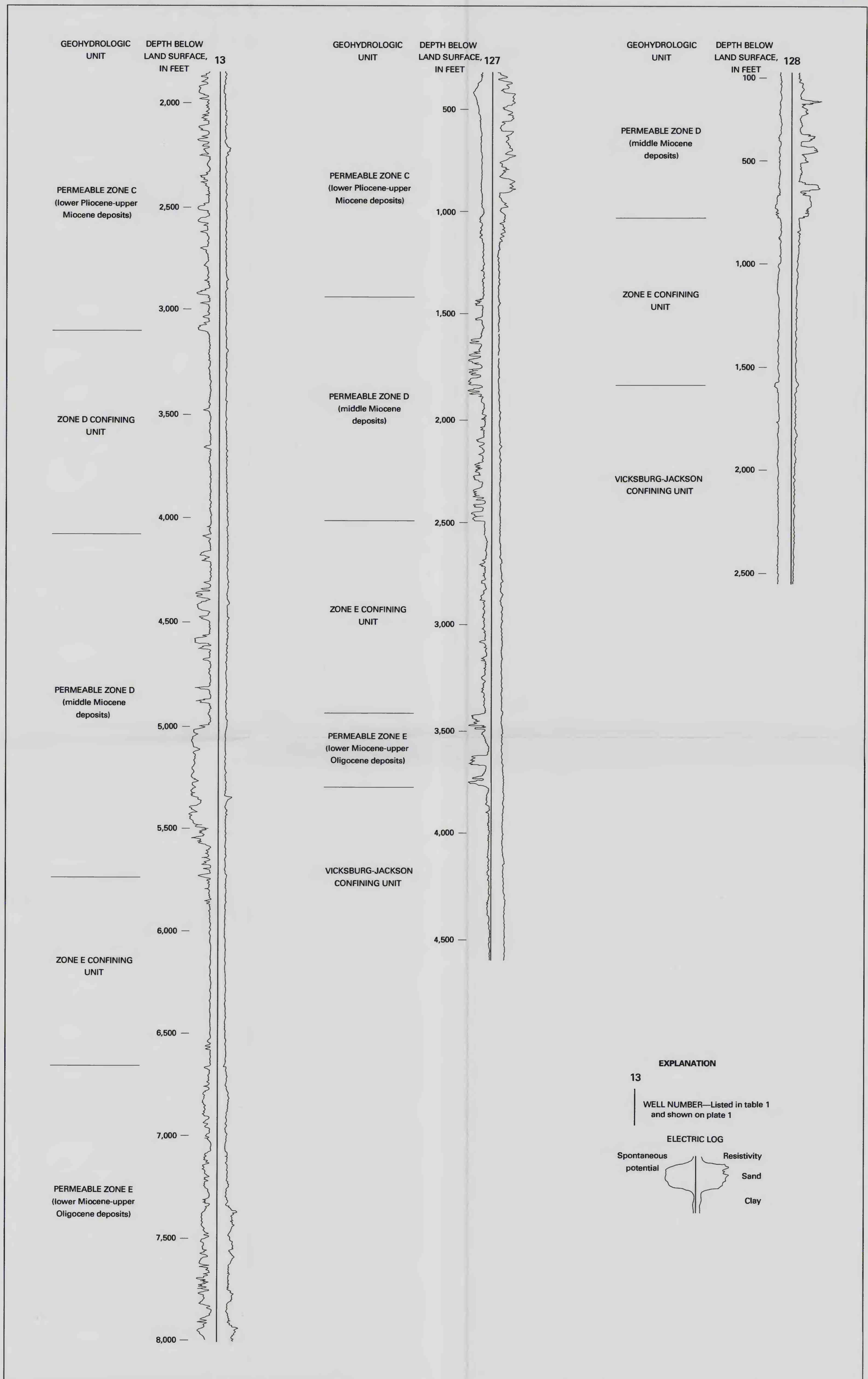
ELECTRIC LOGS SHOWING GEOHYDROLOGIC UNITS IN THE COASTAL LOWLANDS AQUIFER SYSTEM IN SAN PATRICIO, NUECES, AND LIVE OAK COUNTIES, TEXAS
