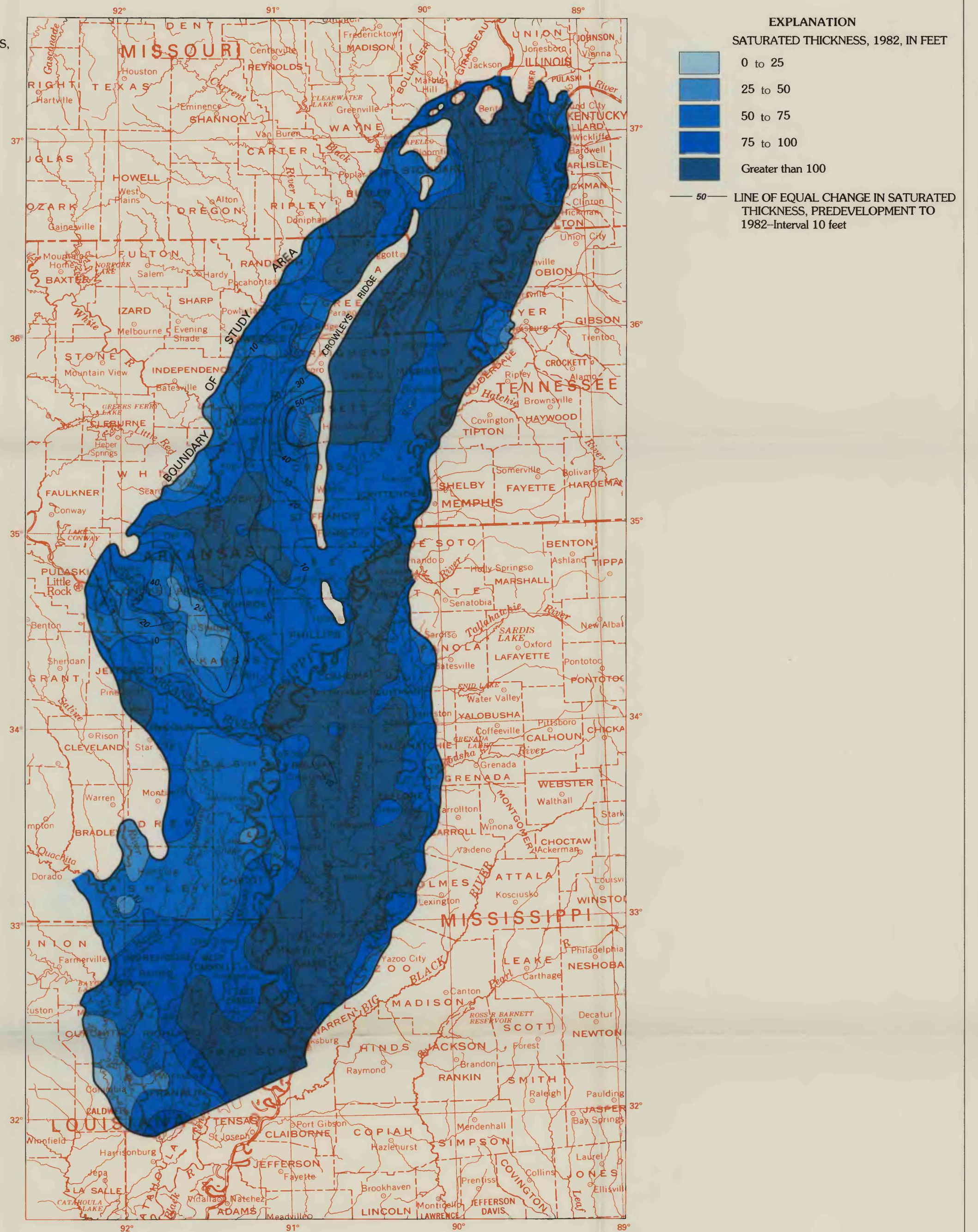
1982 SATURATED THICKNESS AND CHANGE IN SATURATED THICKNESS, PREDEVELOPMENT TO 1982. ESTIMATED FROM SIMULATED HYDRAULIC HEADS
