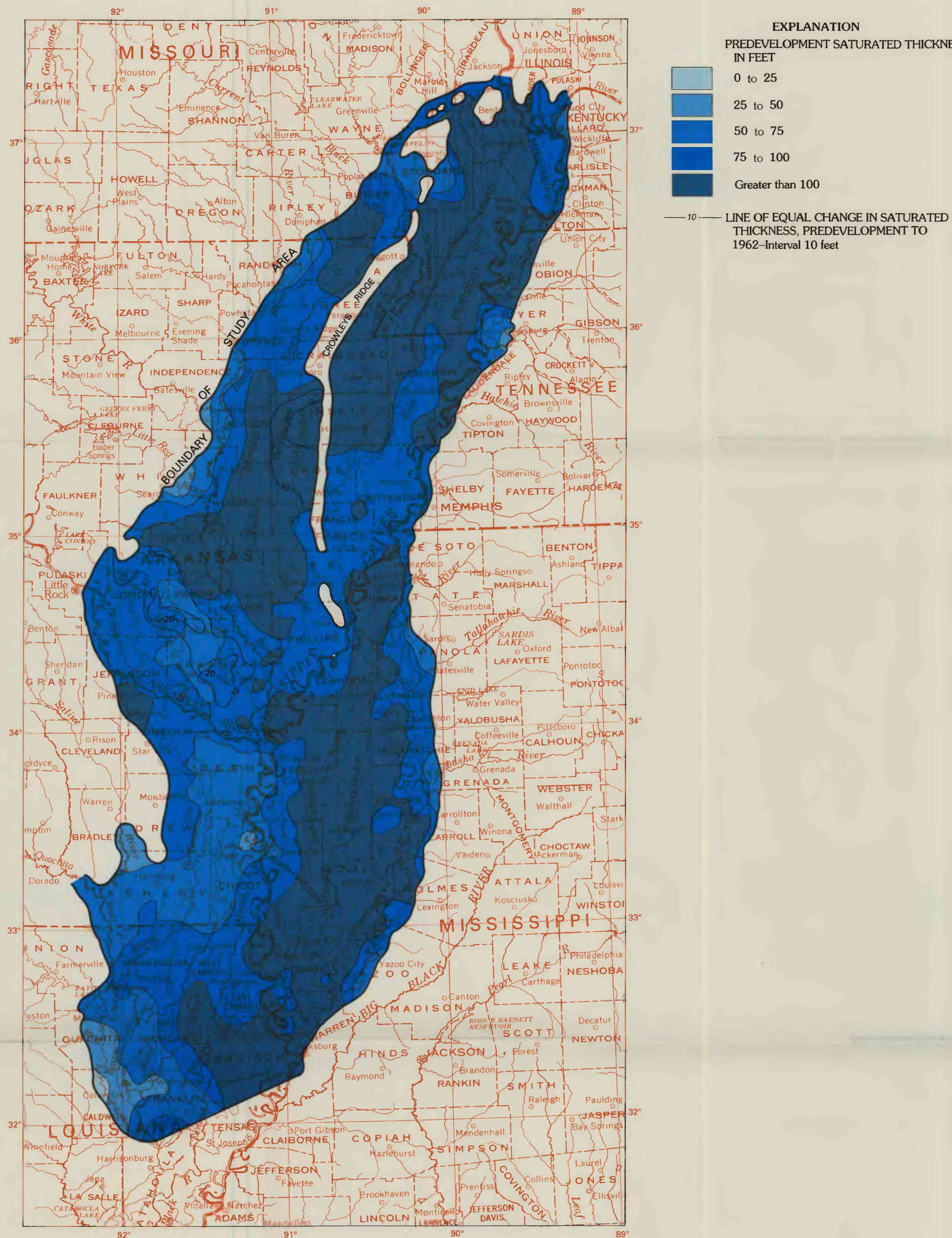
PREDEVELOPMENT SATURATED THICKNESS AND CHANGE IN SATURATED THICKNESS, PREDEVELOPMENT TO 1962. ESTIMATED FROM SIMULATED HYDRAULIC HEADS
