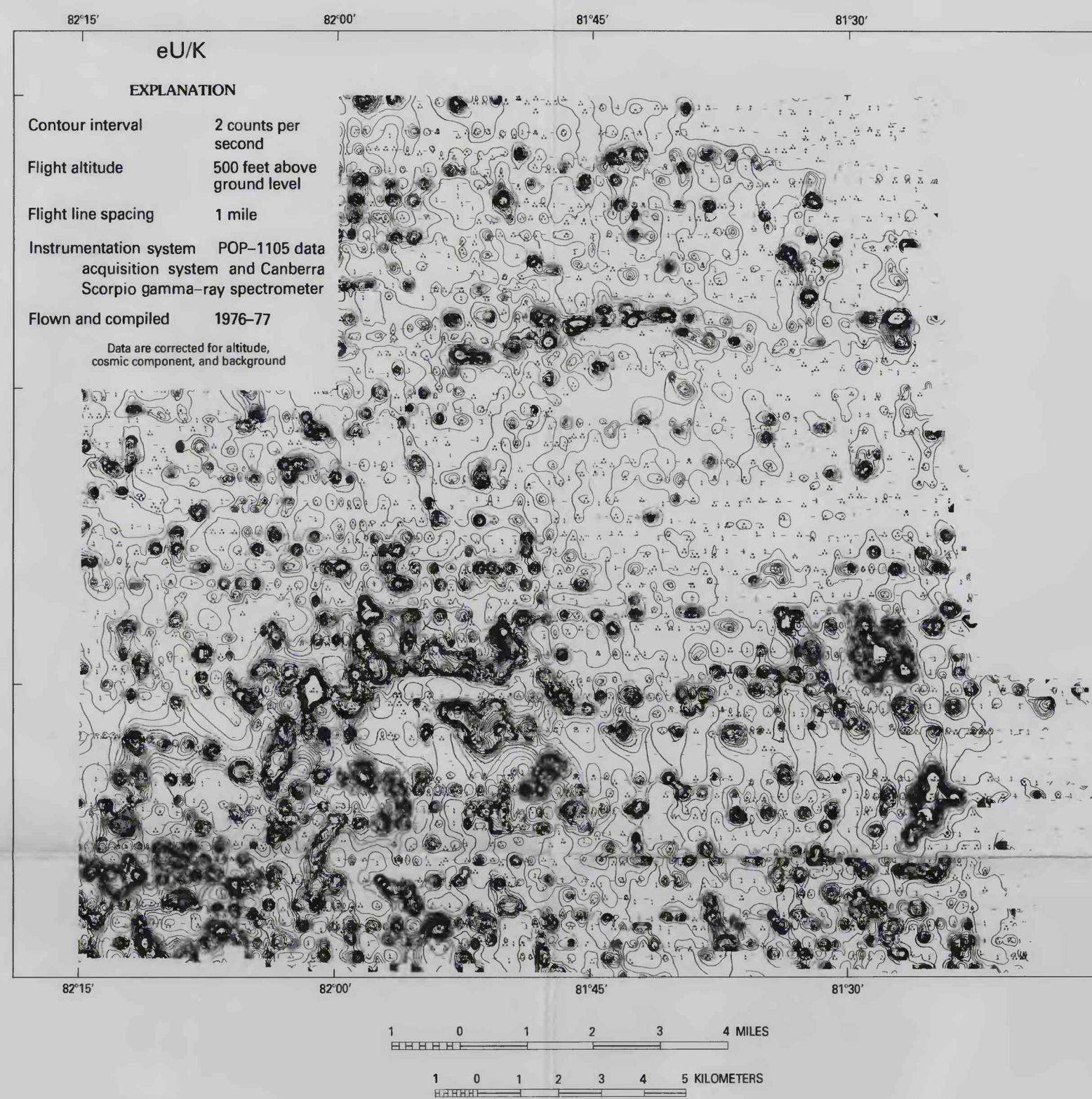
SPECTRAL GAMMA-RAY AERORADIOMETRIC AND RADIOELEMENT RATIO MAPS OF THE JACKSONVILLE AND PORTIONS OF THE VALDOSTA 1° × 2° QUADRANGLES, FLORIDA
