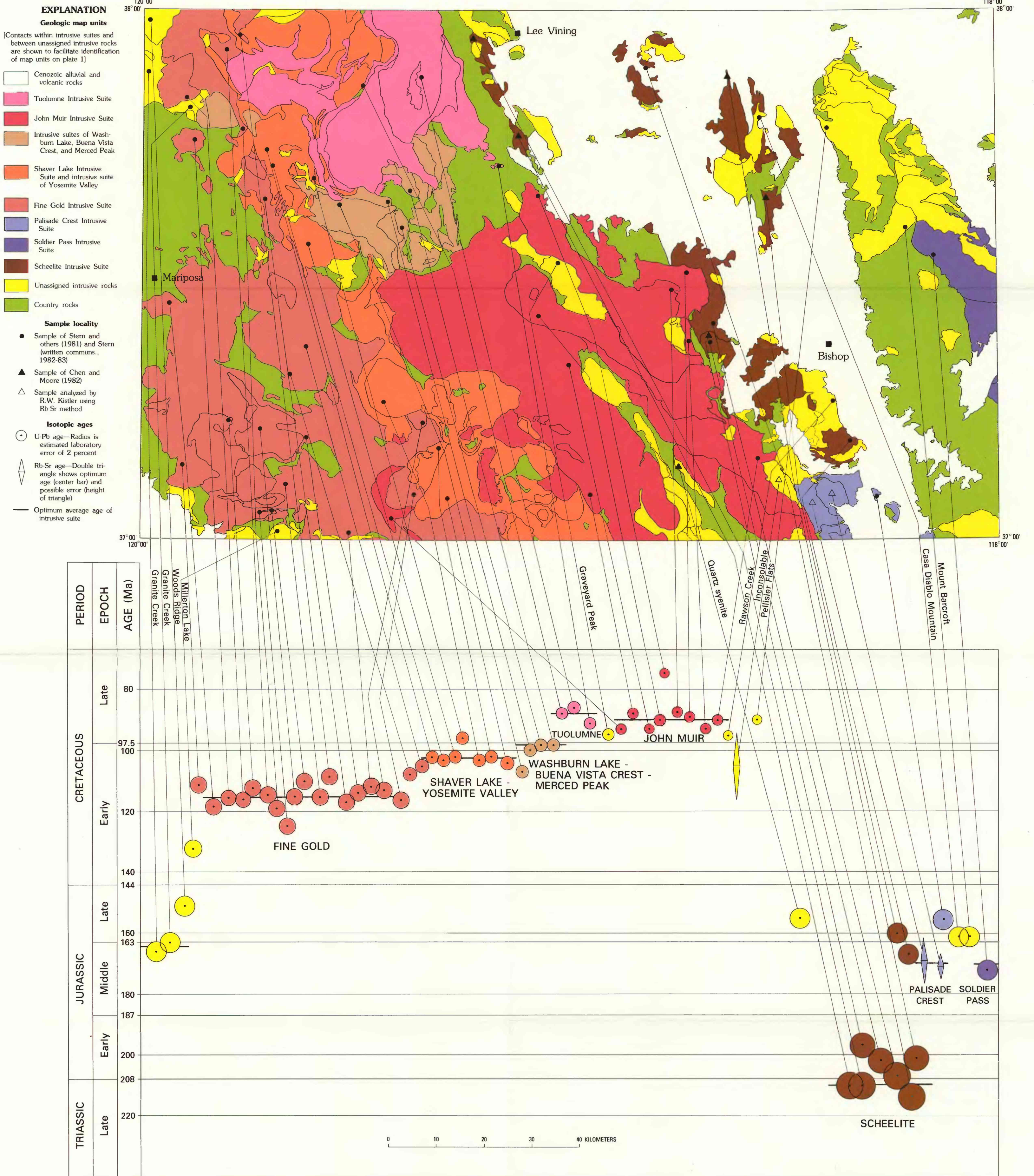
GENERALIZED GEOLOGIC MAP OF THE MARIPOSA 1° BY 2° QUADRANGLE SHOWING SAMPLE LOCALITIES AND CHART SUMMARIZING U-Pb AND Rb-Sr AGES
