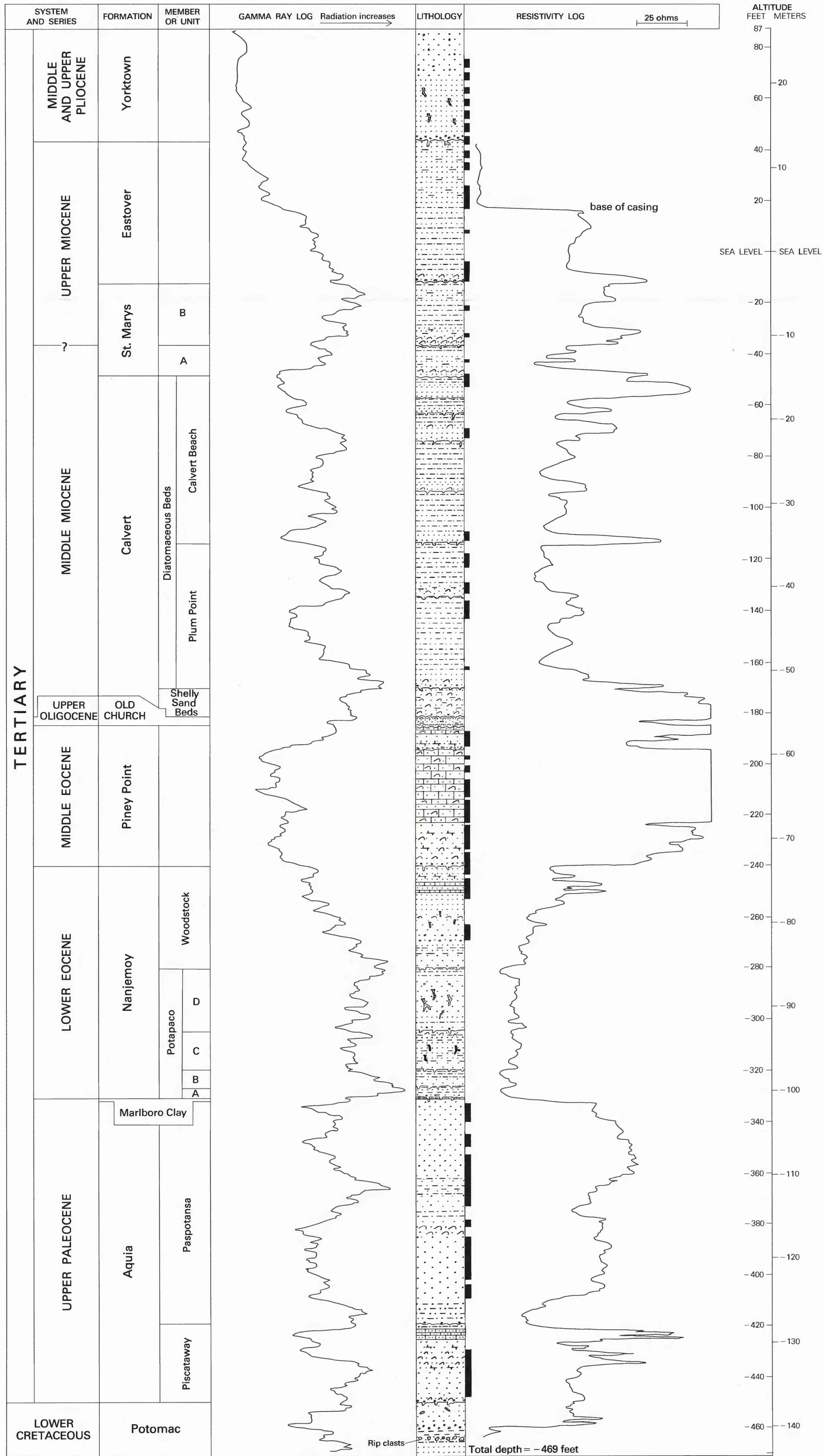
LITHIC, GAMMA RAY, AND ELECTRICAL RESISTIVITY LOGS OF THE HAYNESVILLE CORE HOLES, RICHMOND COUNTY, VIRGINIA
