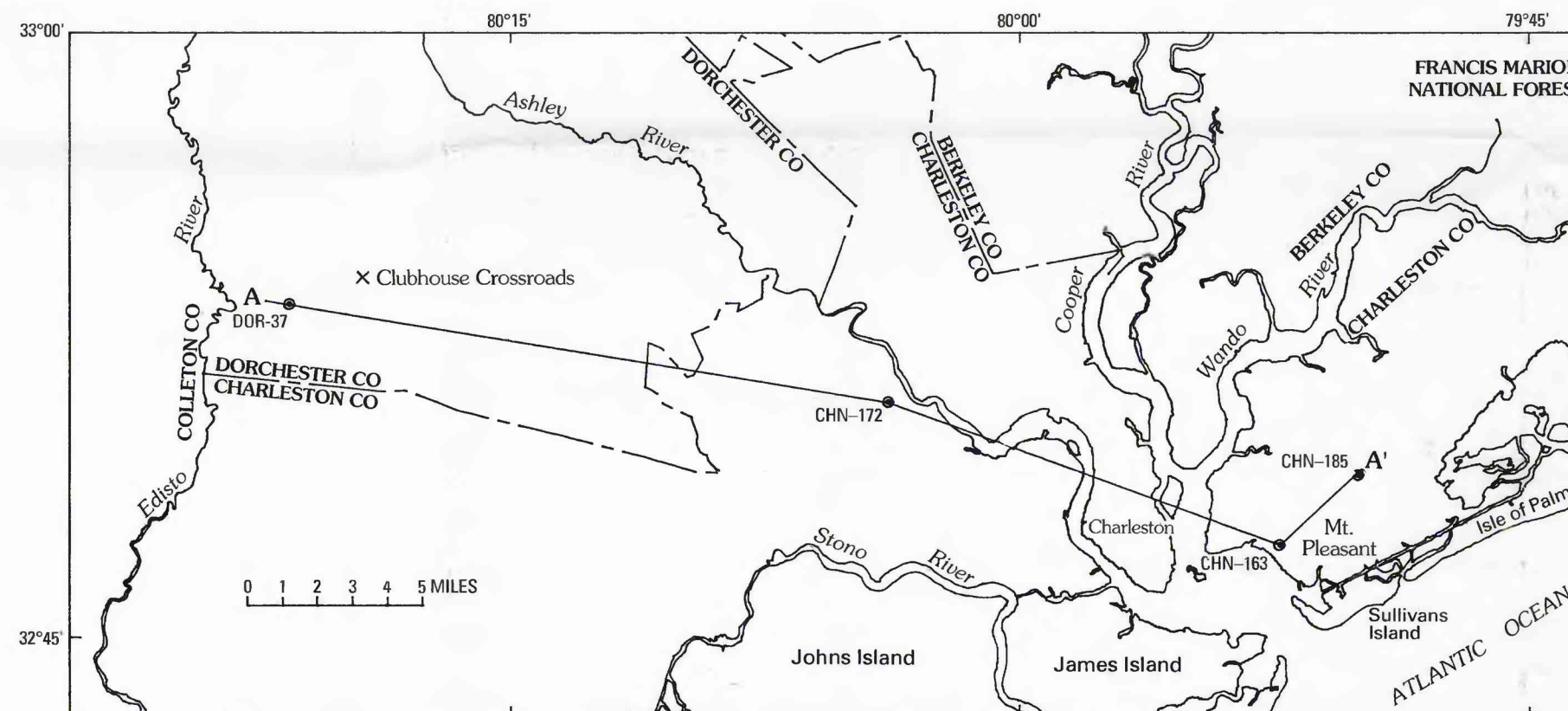
STRATIGRAPHIC CROSS SECTION SHOWING CRETACEOUS UNITS IN SOUTHERN DORCHESTER AND CENTRAL CHARLESTON COUNTIES, SOUTH CAROLINA
