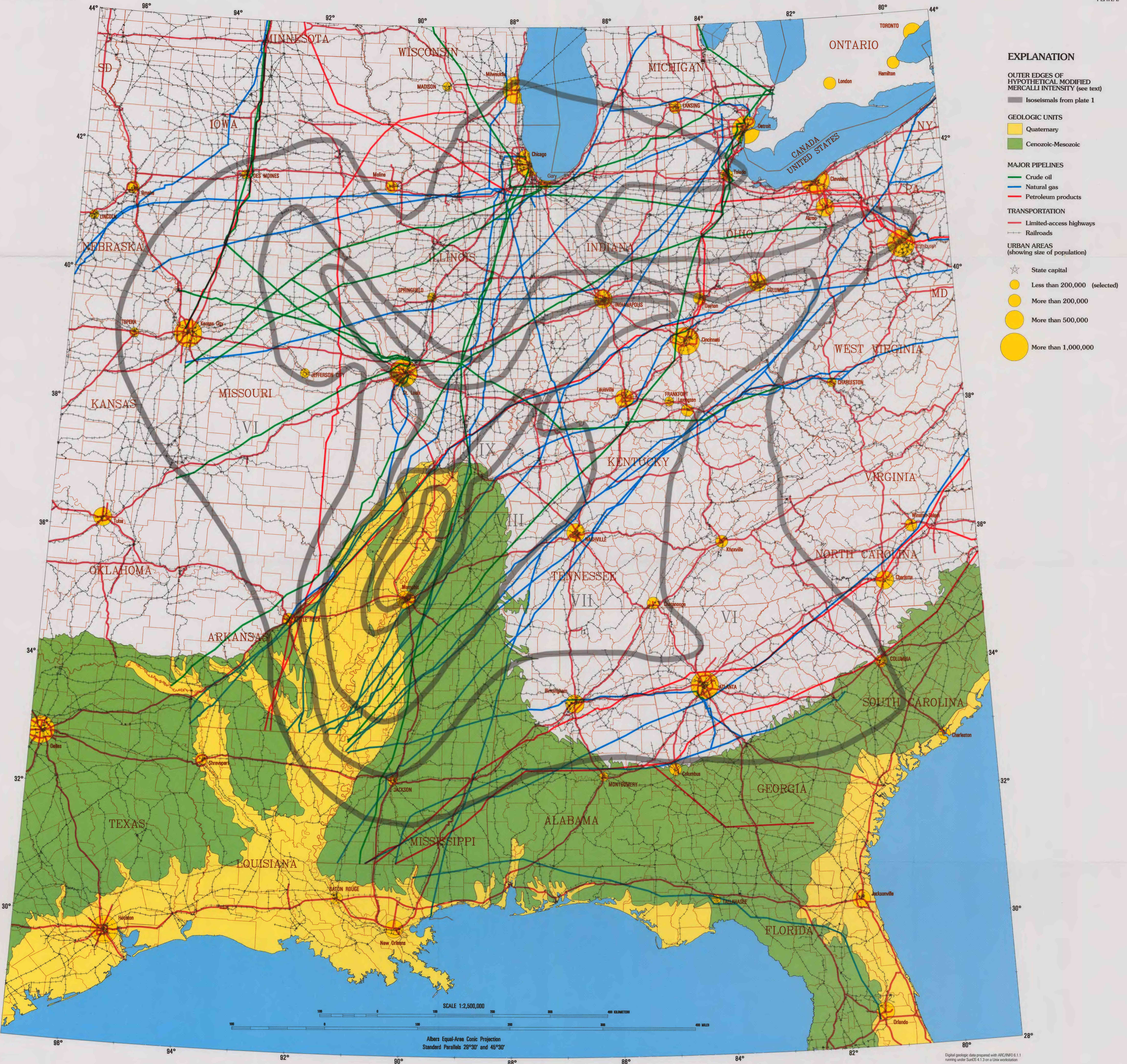
ELEMENTS OF INFRASTRUCTURE AND SEISMIC HAZARD IN THE CENTRAL UNITED STATES—PLATE 2
