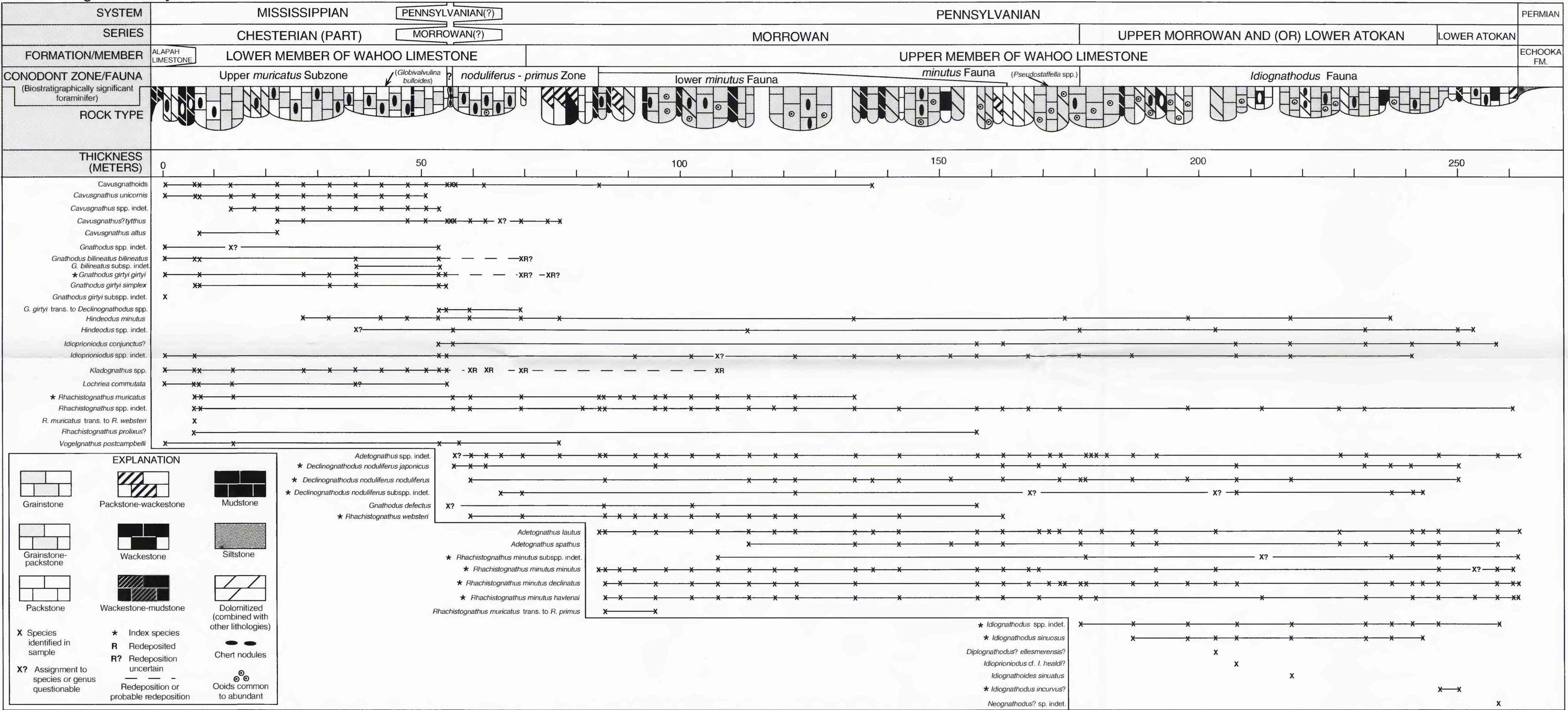
Conodont zones, faunal intervals, and species distribution and lithologies of the Wahoo Limestone in the study section, eastern Sadlerochit Mountains, northeast Brooks Range, Alaska
