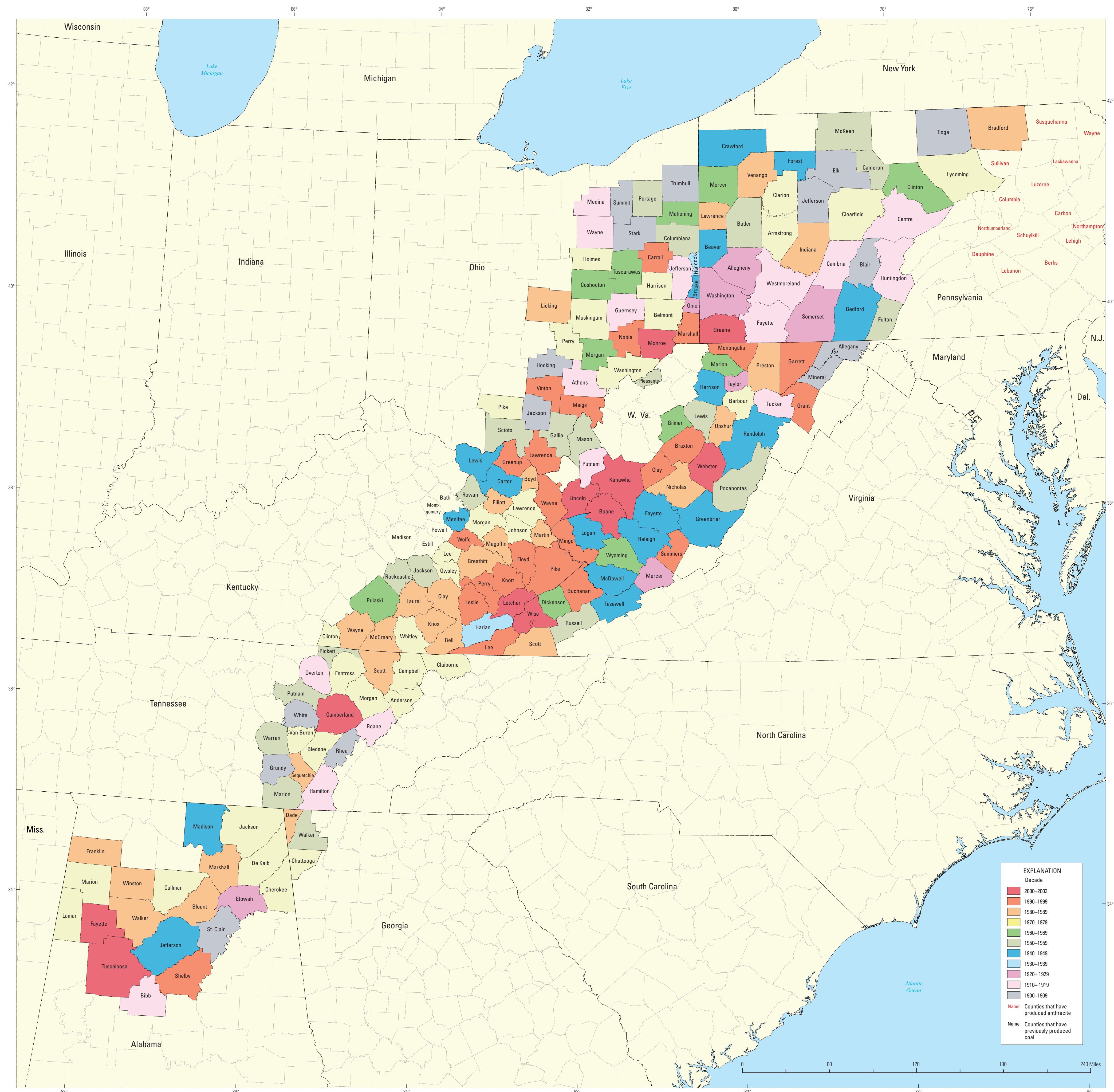
Figure 1. Decade of greatest coal production by county. D.C., District of Columbia; Del., Delaware; Miss., Mississippi; N.J., New Jersey; W. Va., West Virginia.
