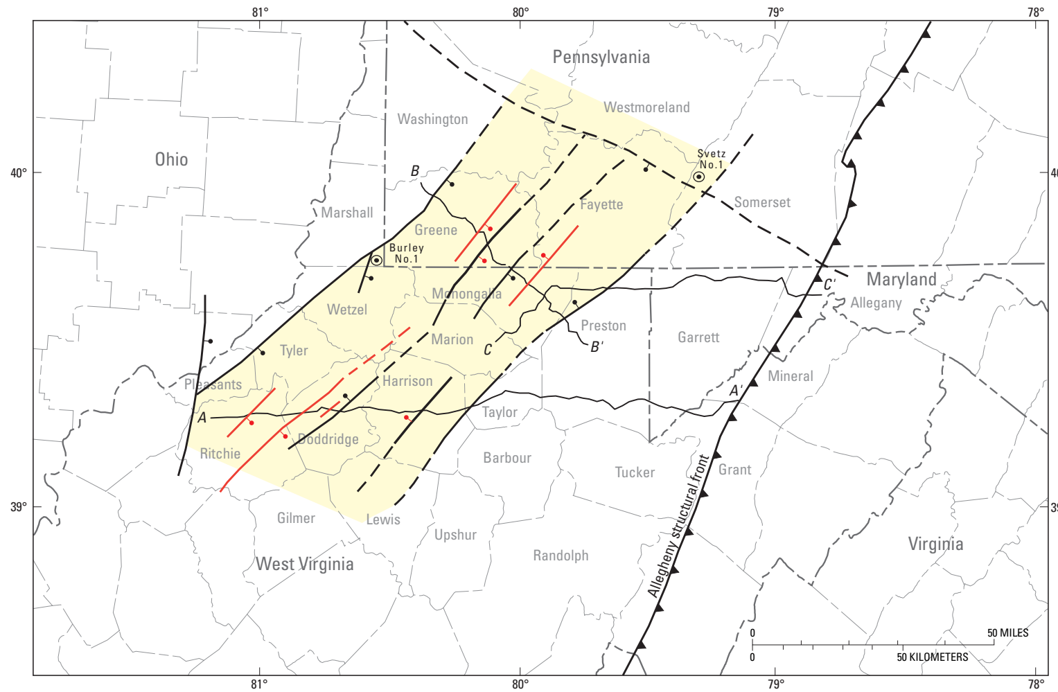
Figure 2.—Location of seismic sections, wells, and major basement faults of the Rome trough. Modified from Shumaker (1996).
