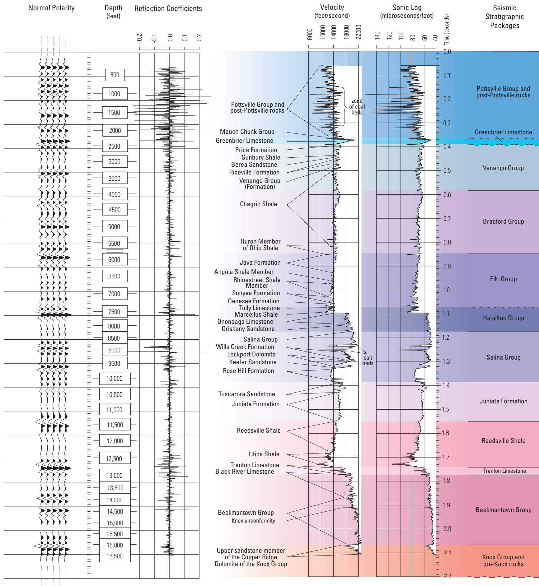
Figure 5.--Synthetic seismogram of the Occidental Petroleum Corporation Burley No. 1 well.
