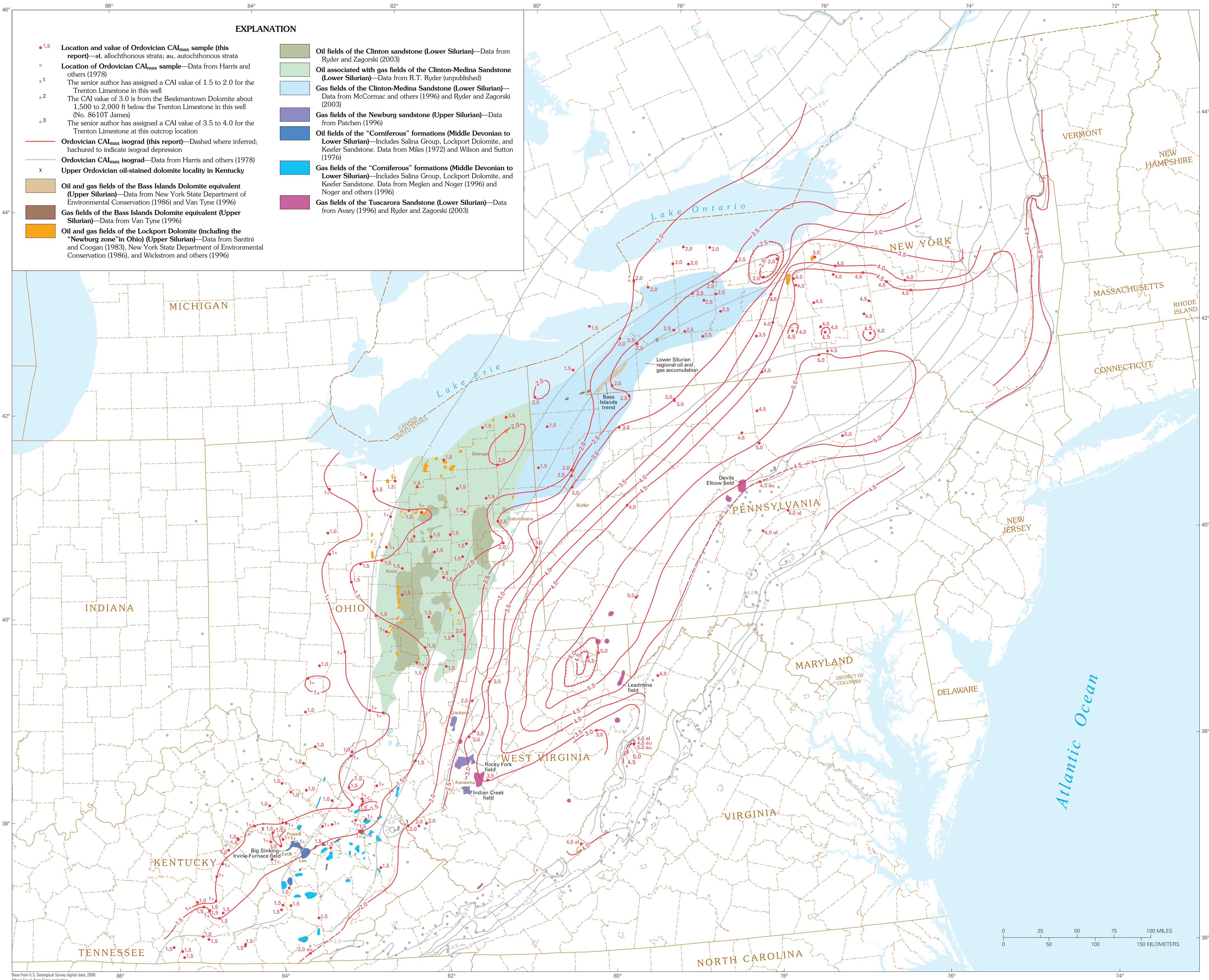
Figure 7. Map showing Ordovician conodont color alteration index ( CAI_{max} ) isograds superimposed on oil and gas fields in Silurian reservoirs.
