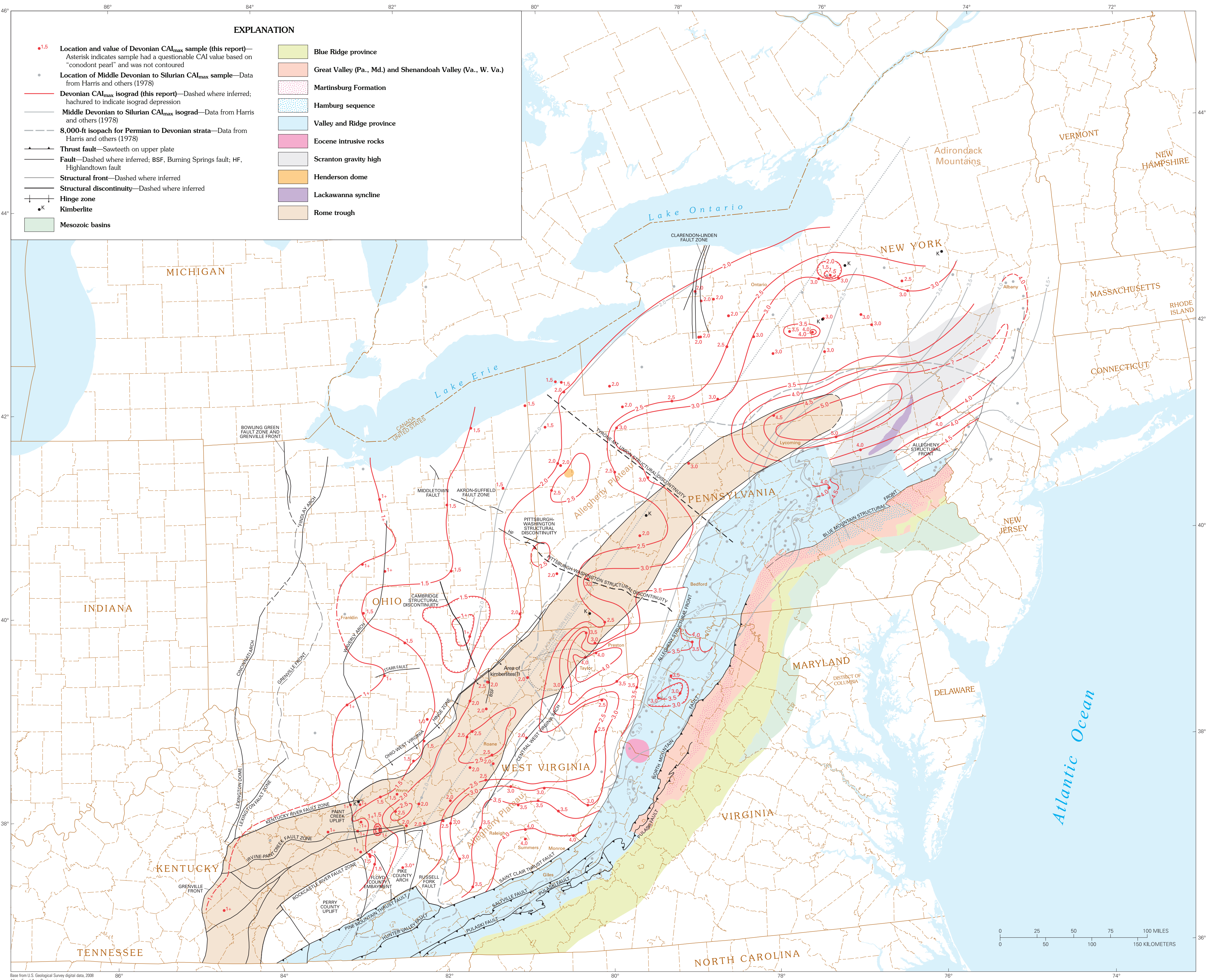
Figure 8. Map showing Devonian conodont color alteration index (CAI max ) isograds superimposed on selected structural features and provinces.
