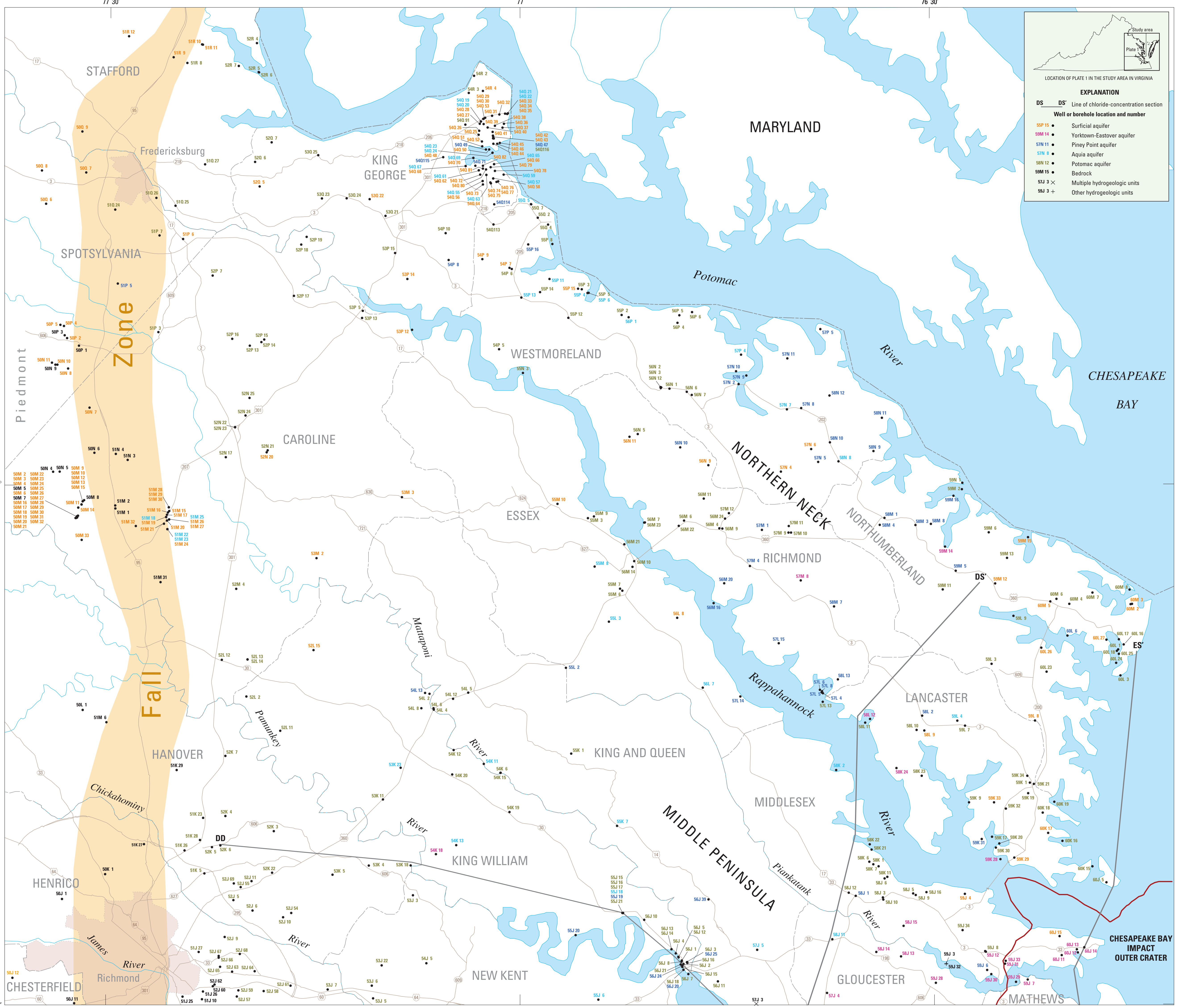
Locations of Sampled Groundwater Wells and Boreholes in the Northern Part of the Virginia Coastal Plain
