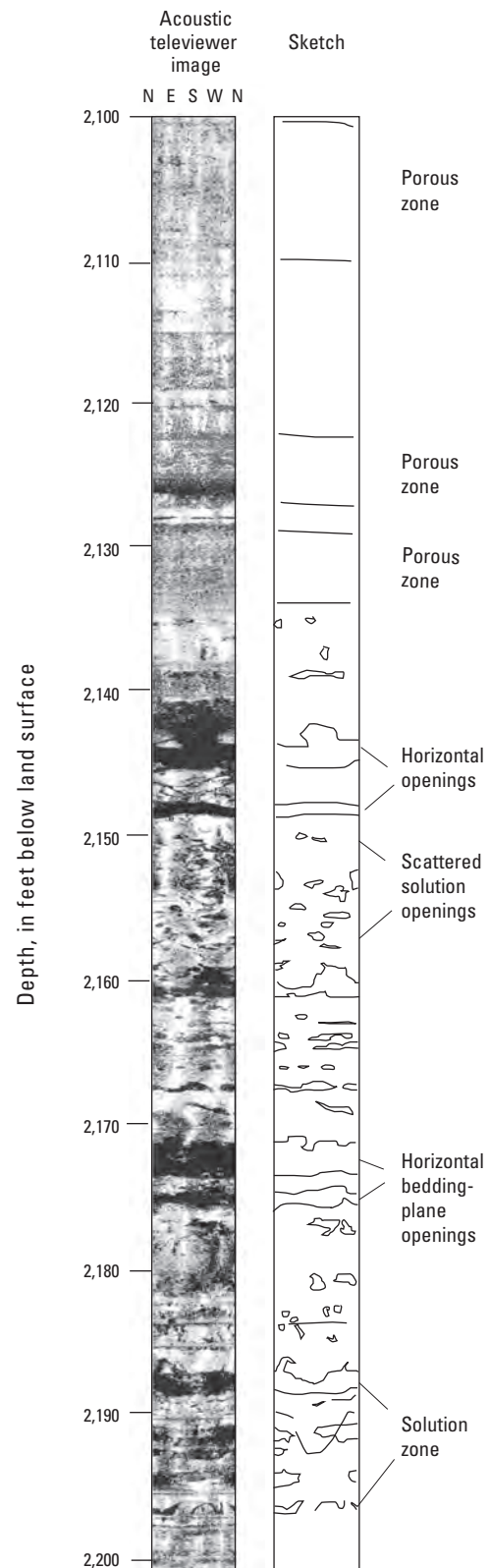
Figure 13. Acoustic televewer image from 2,100 to 2,200 feet showing solution openings formed along bedding planes and in discrete zones near the base of the Oldsmar Formation in test well GA-GLY9, Brunswick, Georgia (well location shown on plate 1).
