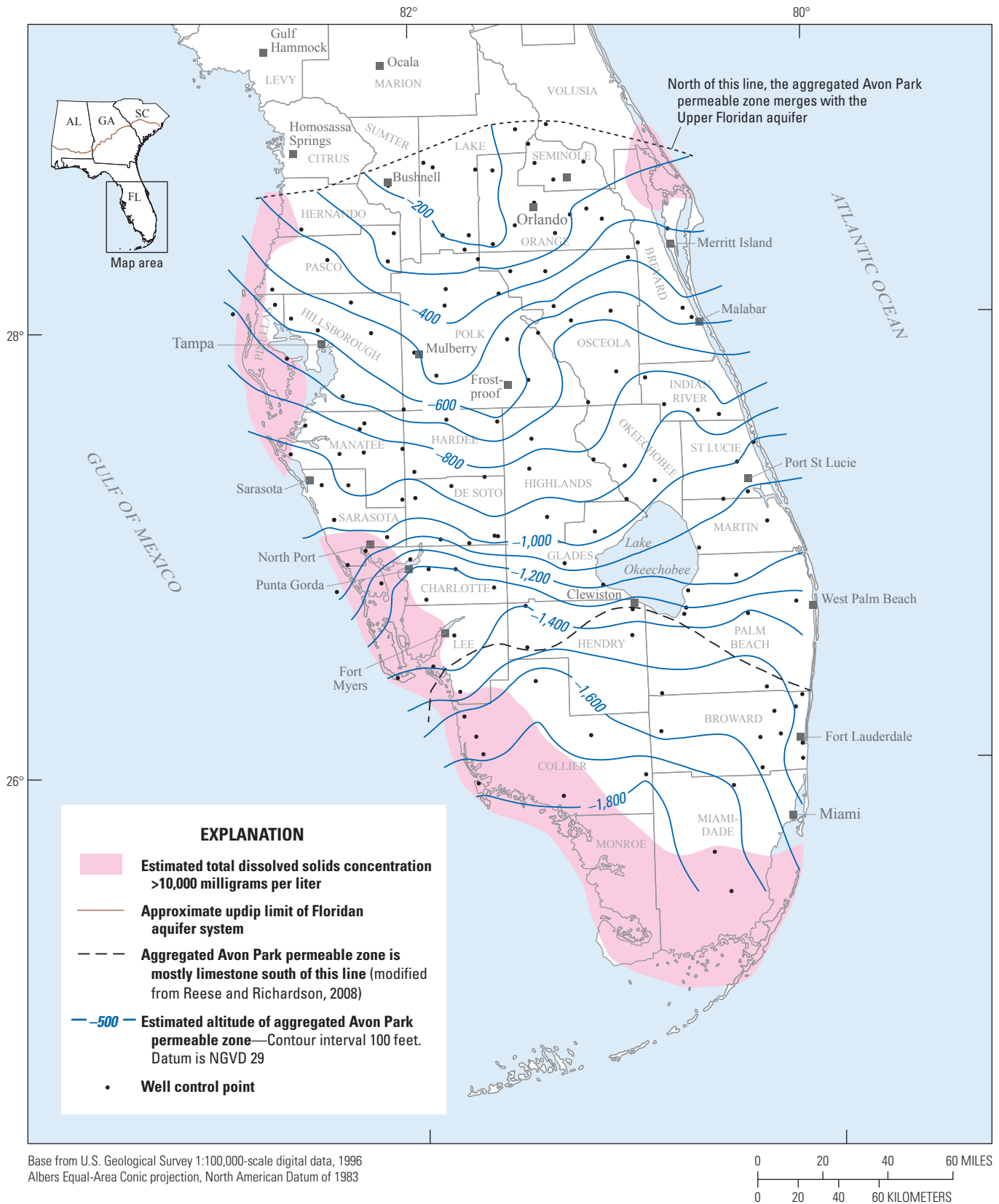
Figure 30. Altitude of the top of the aggregated Avon Park permeable zone and estimated total dissolved solids concentration in central and southern Florida.
