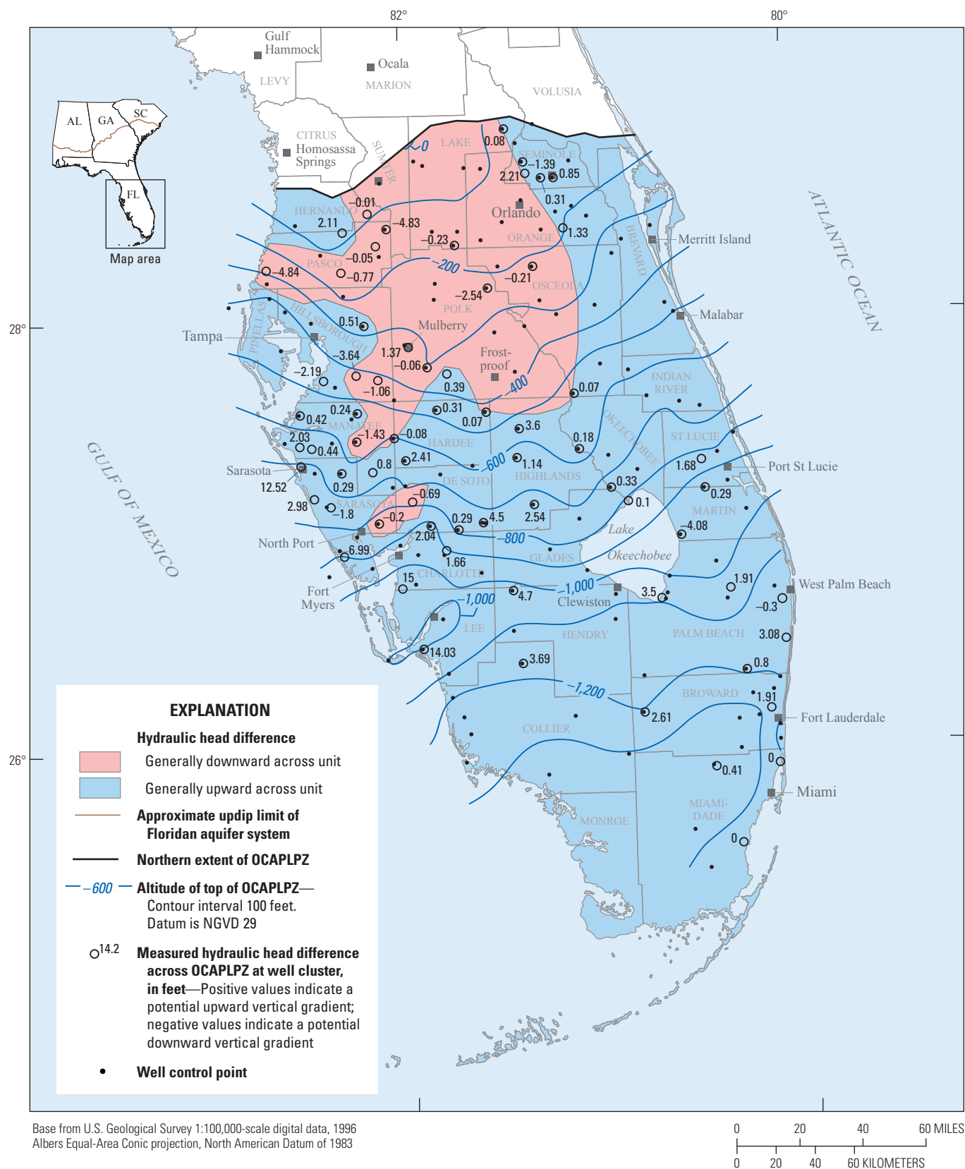
Figure 28. Altitude of the top and hydraulic head difference across the Ocala-Avon Park lower permeability zone (OCAPLPZ) in central and southern Florida.
