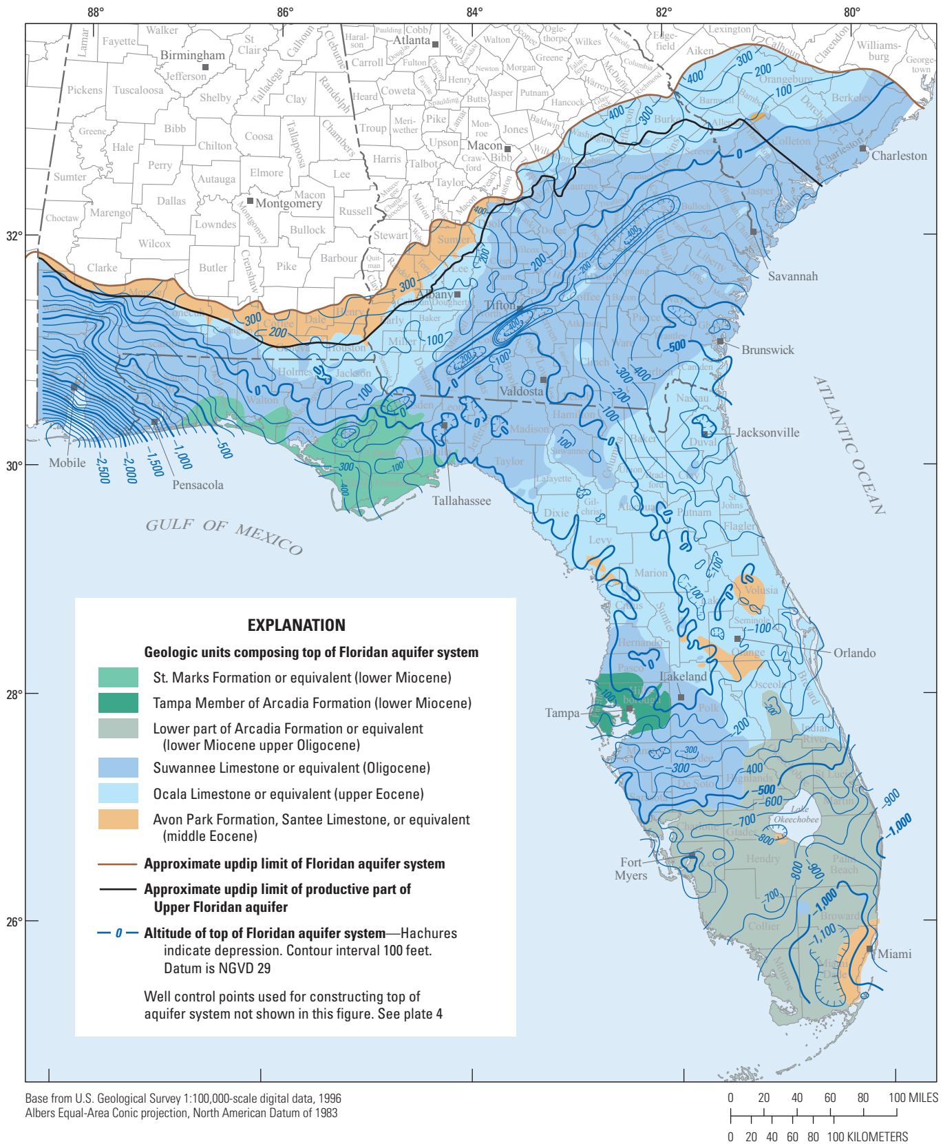
Figure 22. Generalized altitude of the top of the Floridan aquifer system, southeastern United States (see plate 4 for more detail).
