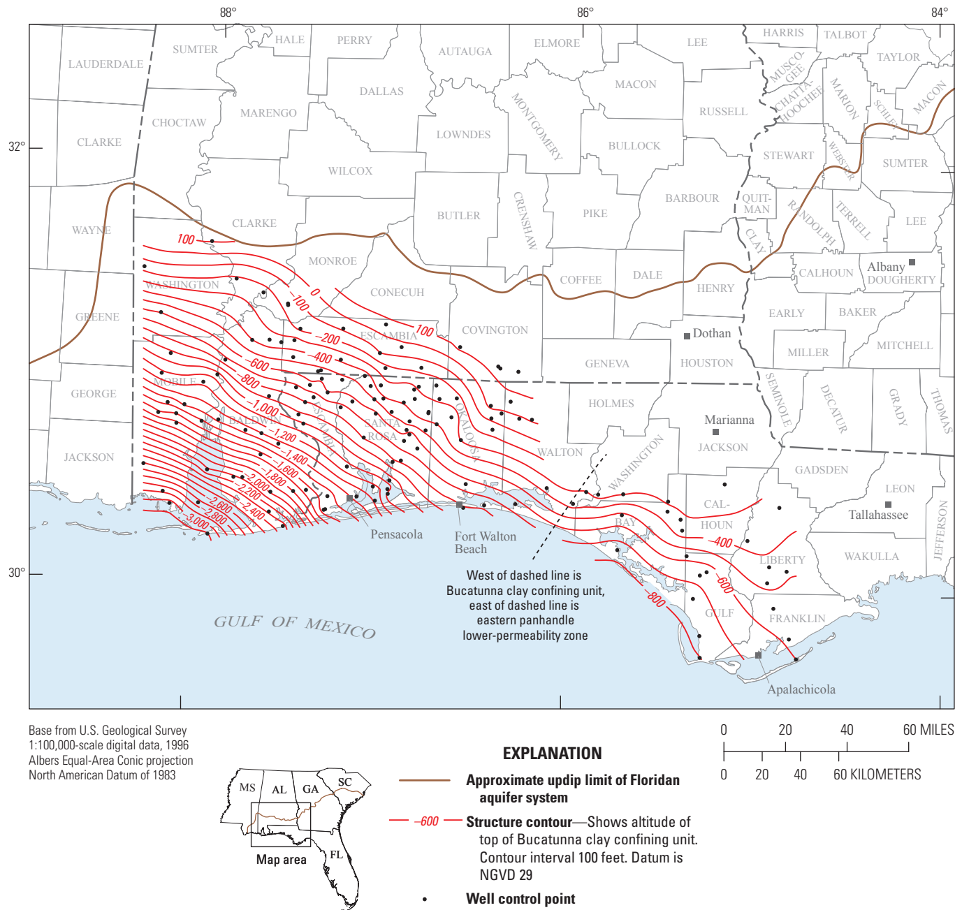
Figure 43. Altitude of the top of the Bucatanunna clay confining unit, western panhandle Florida and southwestern Alabama.
