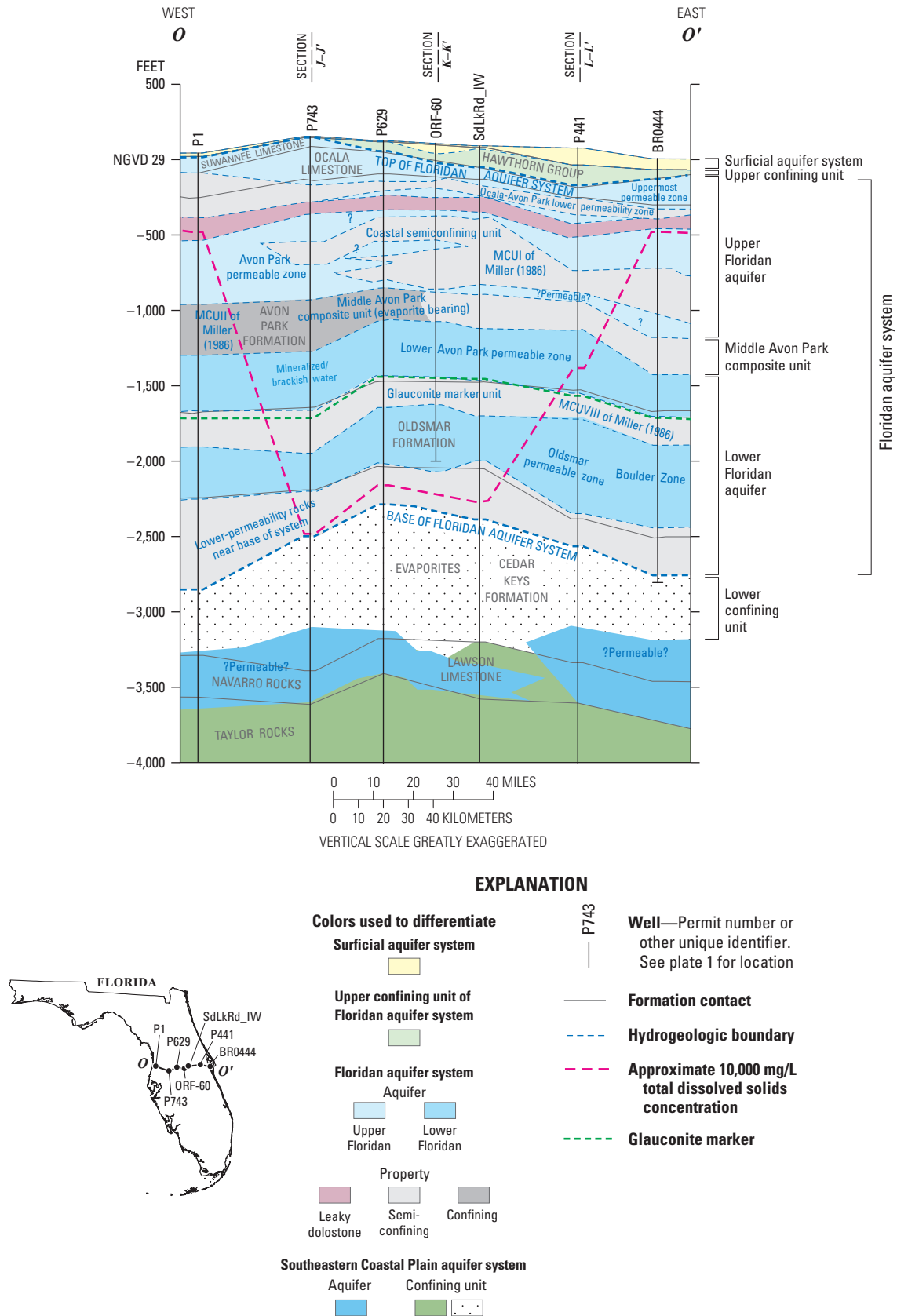
Figure 40. Generalized hydrogeologic cross section O-O' from Hernando County, Florida, to Brevard County, Florida (see plate 21 for more detail).
