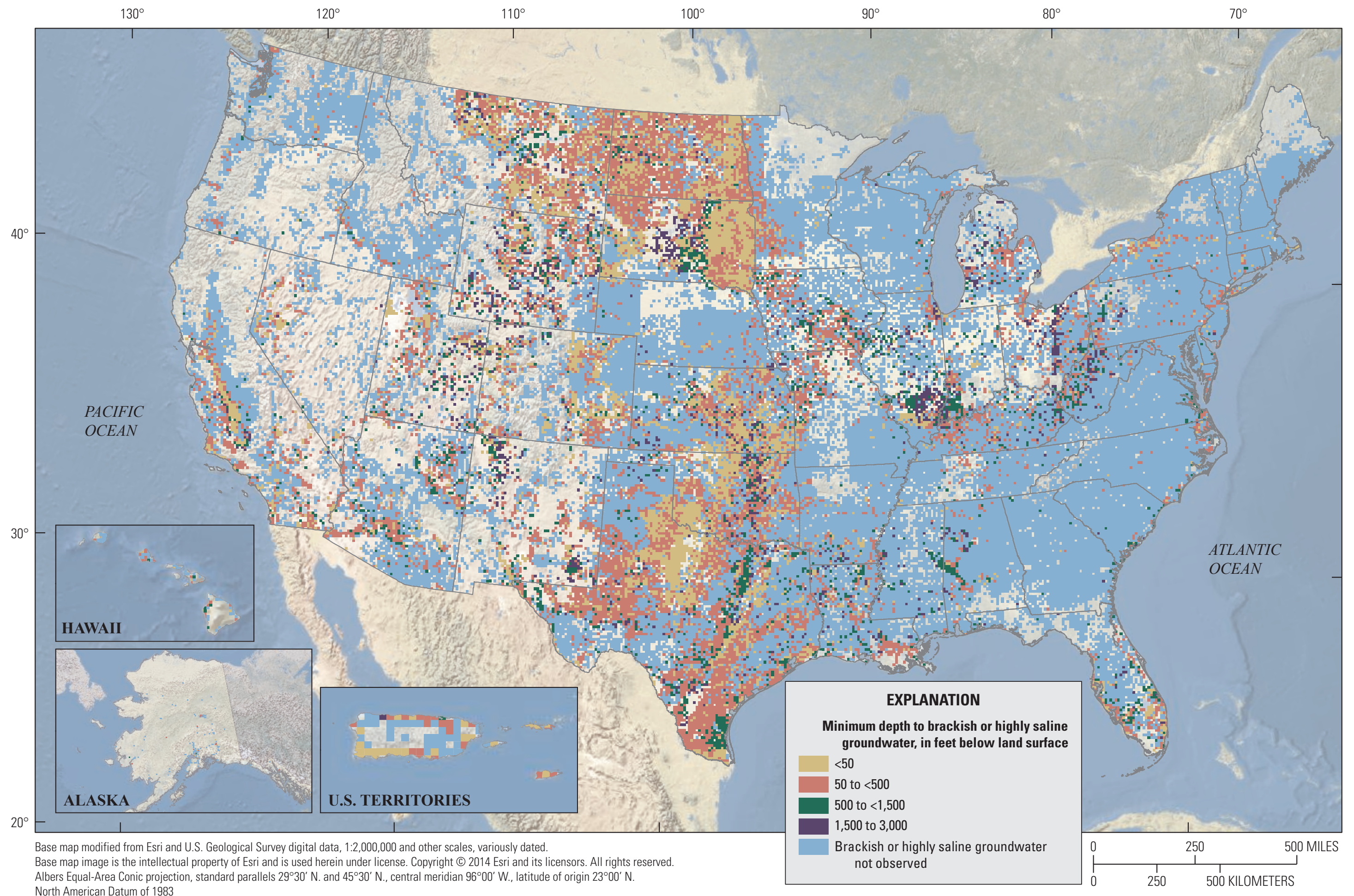
Figure 10. Observed minimum depth to brackish or highly saline groundwater in the United States and selected U.S. territories.
