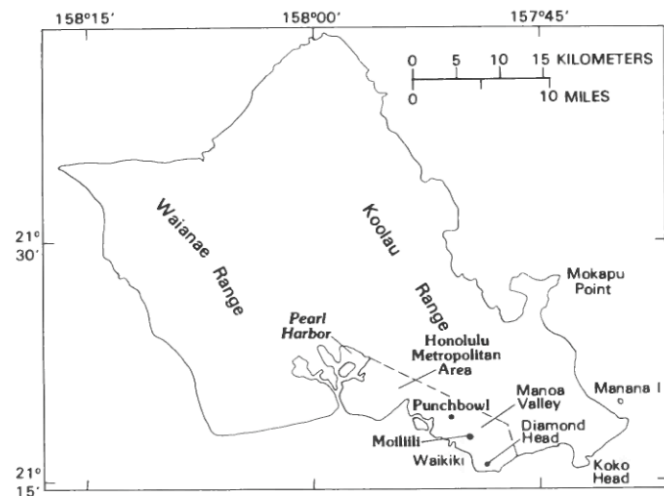
FIGURE 22.17.—The Island of Oahu. The Waiānae and Koolau Ranges are each deeply eroded shield volcanoes more than 2 million years old. The most recent eruptions on Oahu originated at vents located between Koko Head and Manana Island.
