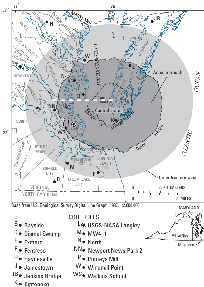
Figure A1. Regional map showing the location of the Chesapeake Bay impact structure, the USGS-NASA Langley corehole at Hampton, Va., and some other coreholes in southeastern Virginia. White dashed line indicates approximate location of schematic cross sections in figure A7. Locations of the central crater and outer margin are from Powars and Bruce (1999). The extent of the outer fracture zone (light gray) is based on Powars (2000) and Johnson and others (2001); the eastern part is speculative. Illustration modified from Powars, Johnson, and others (2002) and Edwards and Powars (2003).
