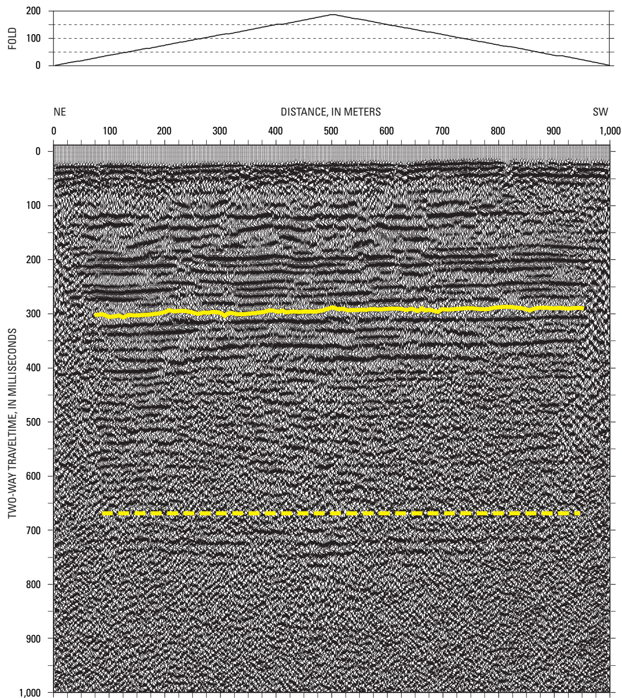
Figure 16. Time-distance seismic-reflection image for the Langley profile. The lower highlighted boundary (at about 670 ms) is between crystalline basement rocks (the Langley Granite in the USGS-NASA Langley core) and overlying preimpact sediments. The upper highlighted boundary (at about 300 ms) is between preimpact and synimpact sediments and overlying postimpact sediments. The seismic sources were energetic enough to provide signals from depths of about 1 km (0.6 mi) along part of the seismic profile with a fold of only 1.
