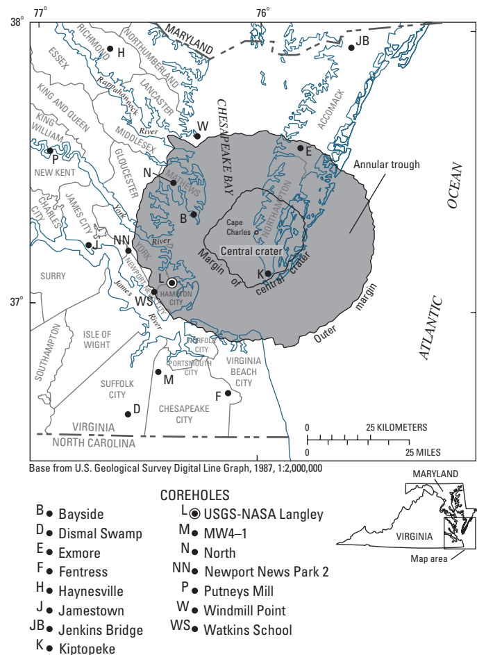
Figure I1. Regional map showing the location of the Chesapeake Bay impact structure, the USGS-NASA Langley corehole at Hampton, Va., and some other coreholes in southeastern Virginia. Locations of the central crater and outer margin are from Powars and Bruce (1999). Illustration modified from Powars, Johnson, and others (2002) and Edwards and Powars (2003).
