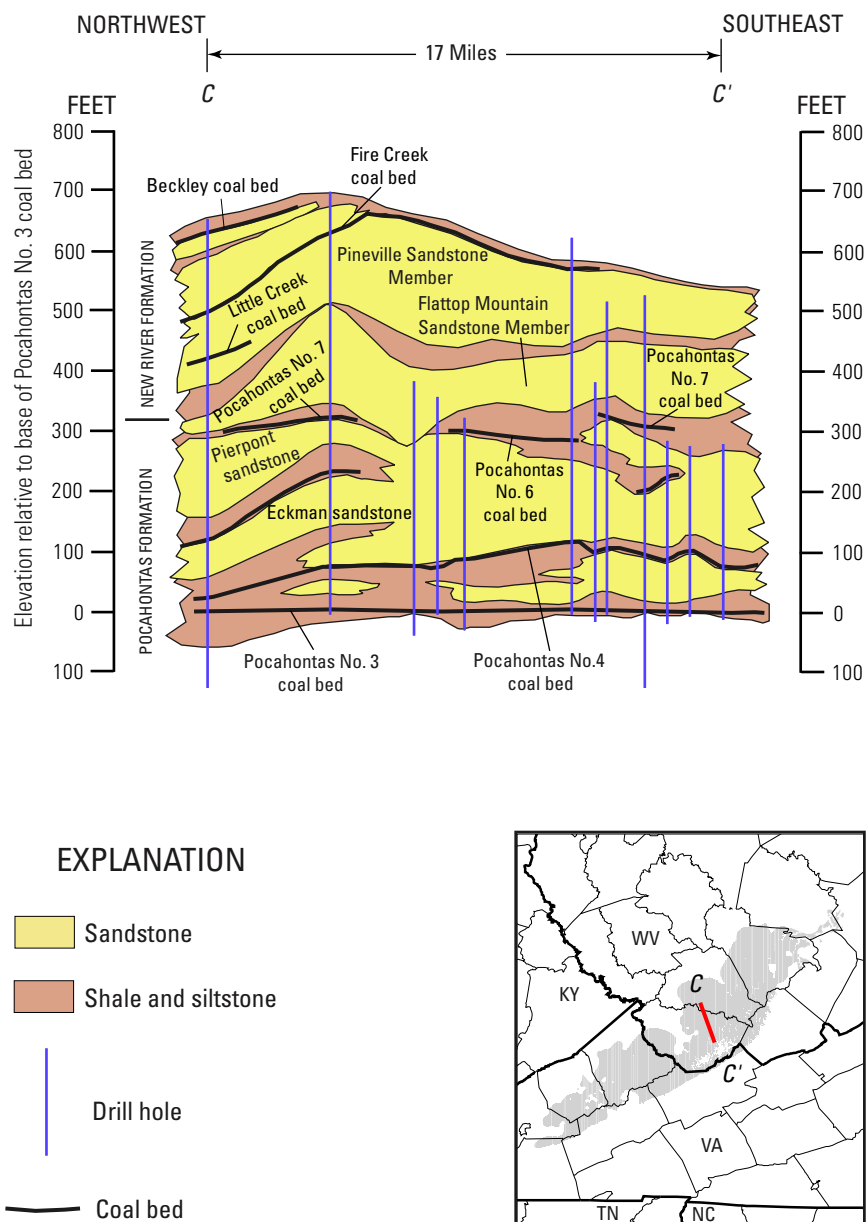
Figure 12. Cross section C-C' (fig. 7) trending northwest to southeast (cross strike) showing the unconformity at the base of the Pineville Sandstone Member of the New River Formation in West Virginia. The Eckman and Pierpont sandstones are informally named units. See figure 2 for county names. Vertical exaggeration X30.
