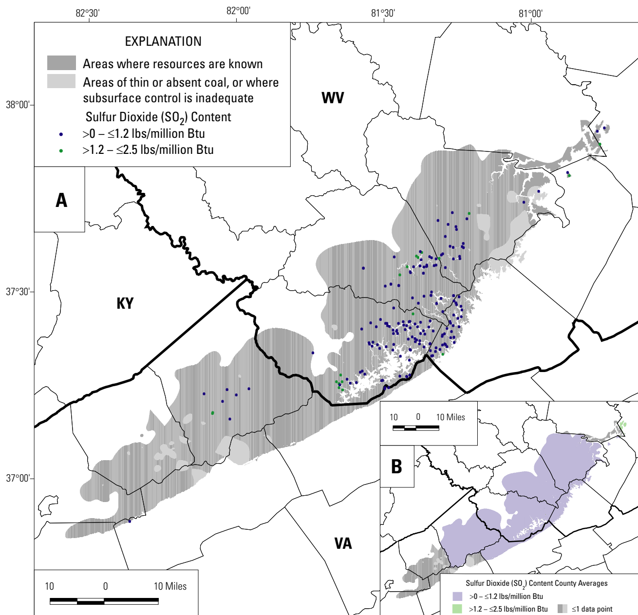
Figure 17. Maps showing sulfur-dioxide ( \text{SO}_2 ) content (lbs/million Btu) of the Pocahontas No. 3 coal bed in Virginia and West Virginia. Map A shows \text{SO}_2 contents of 194 geochemical samples for which records are publicly available and located by latitude and longitude (Appendix 2). Map B shows county averages for \text{SO}_2 contents using all 194 records in the geochemical database, including those that are located only to a county level; \text{SO}_2 values range from 0.56 to 1.66 lbs/million Btu with a mean value of
