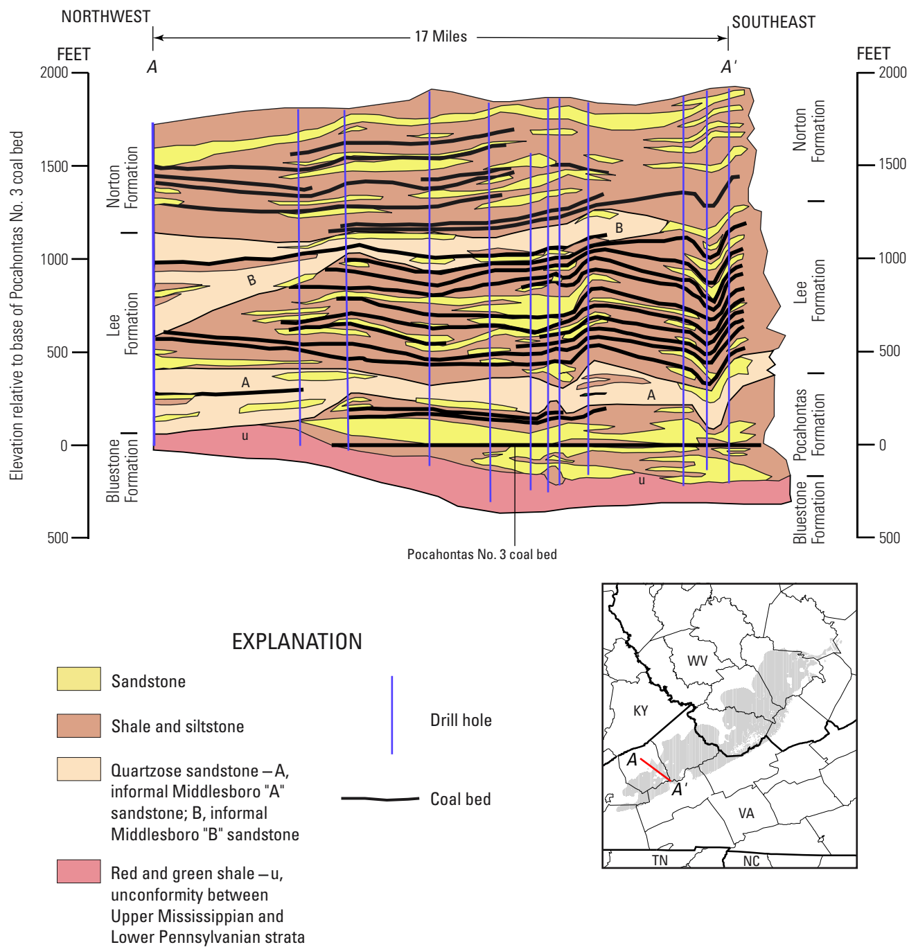
Figure 10. Cross section A-A' (fig. 7) trending northwest to southeast (cross strike) showing the unconformity (u) between the Upper Mississippian and Lower Pennsylvanian strata in southwestern Virginia. See figure 2 for county names. Vertical exaggeration X30.
